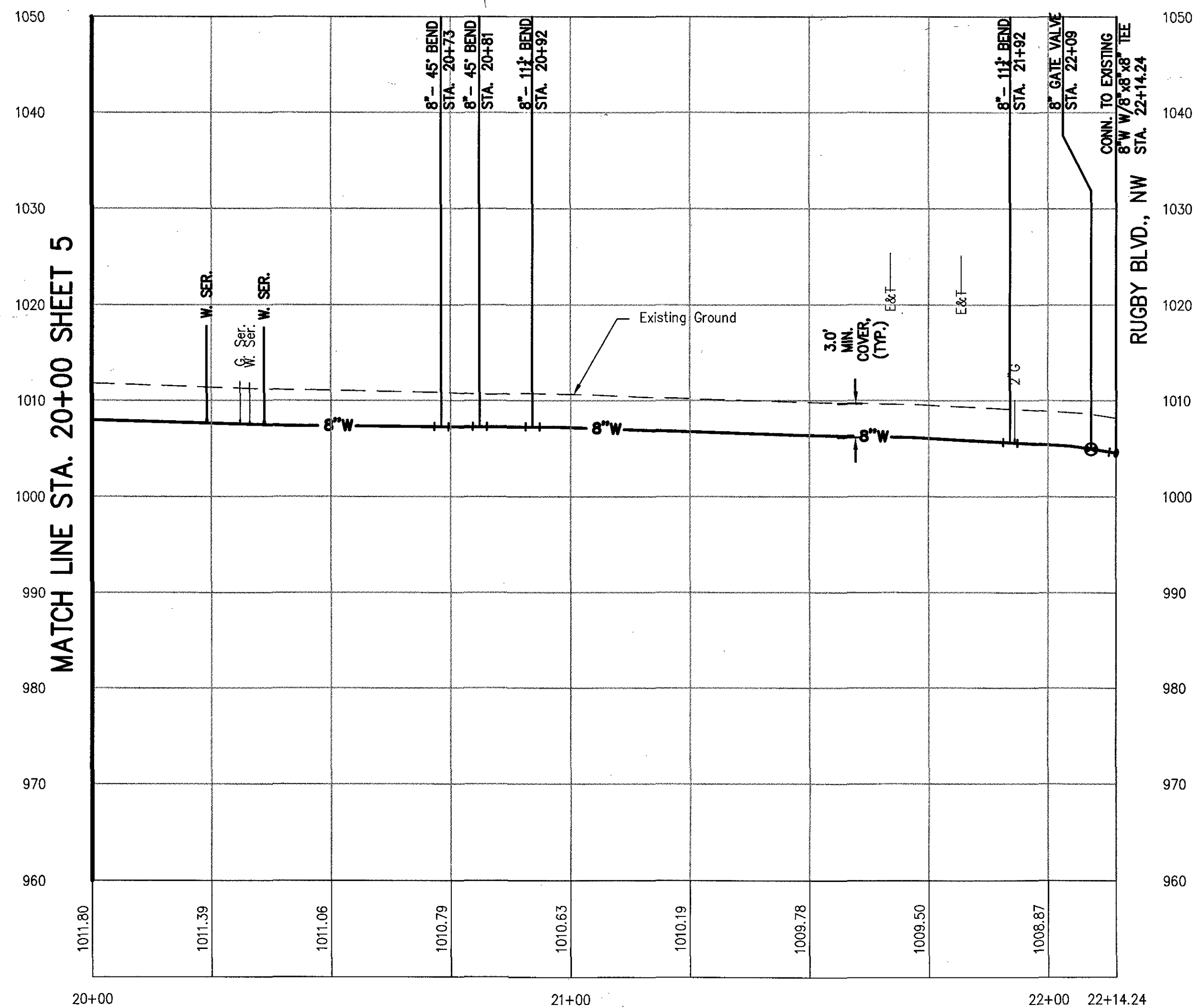
8 INCH WATER MAIN – GRAYSON AVE. PROFILE
