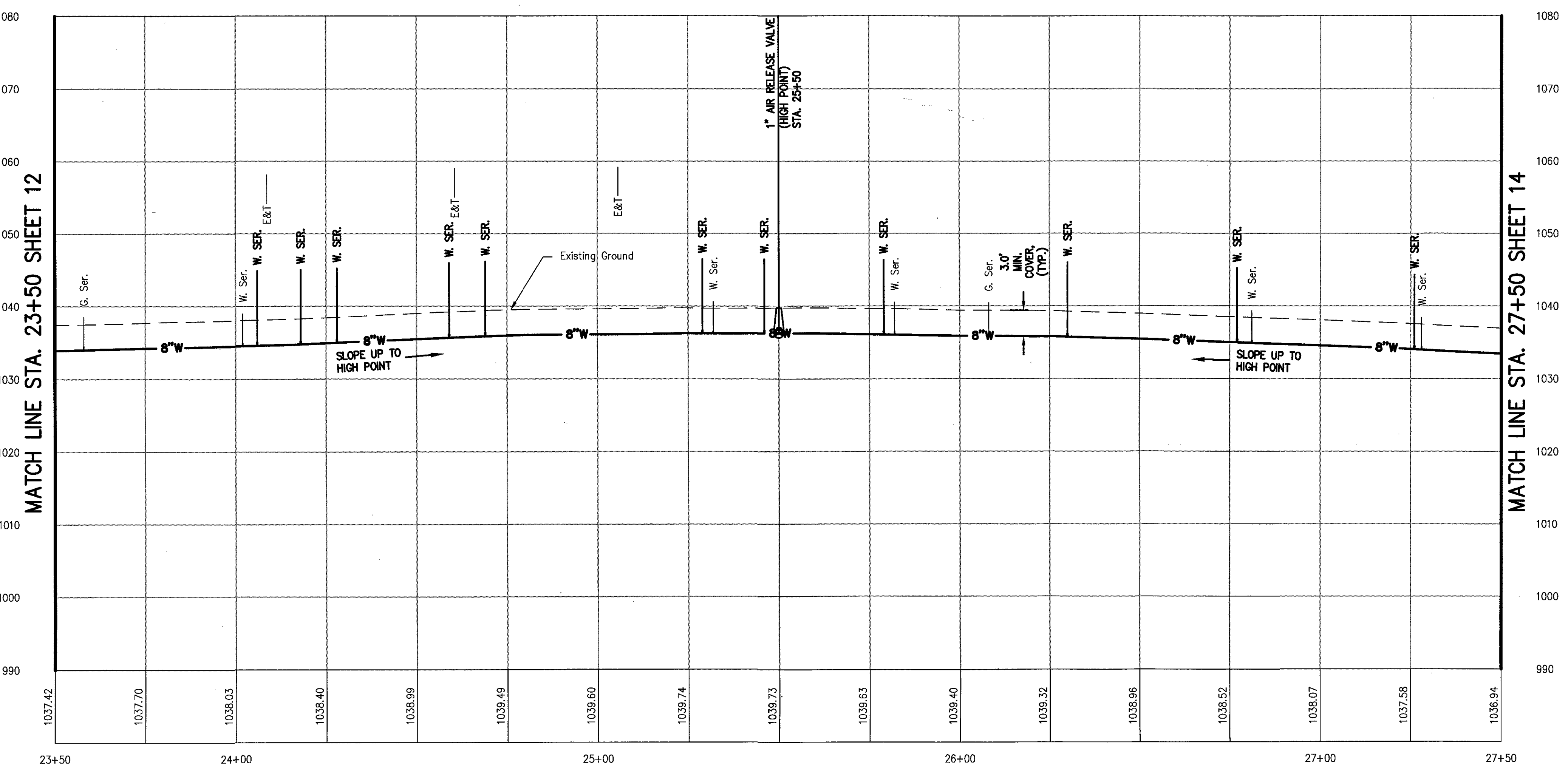
8 INCH WATER MAIN – SYRACUSE AVE. PROFILE
