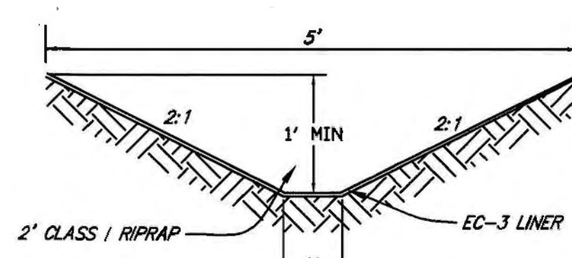
TYPE "B" DITCH NO SCALE
