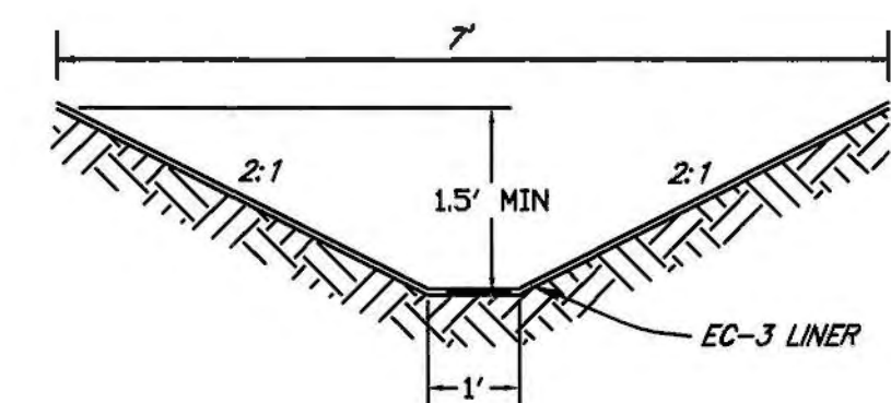
TYPE "A" DITCH NO SCALE
