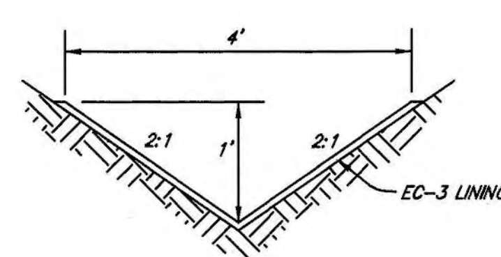
TYPE "C" DITCH NO SCALE
