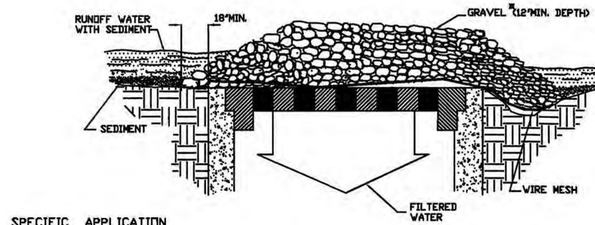
(IP) GRAVEL AND WIRE MESH DROP INLET SEDIMENT FILTER
