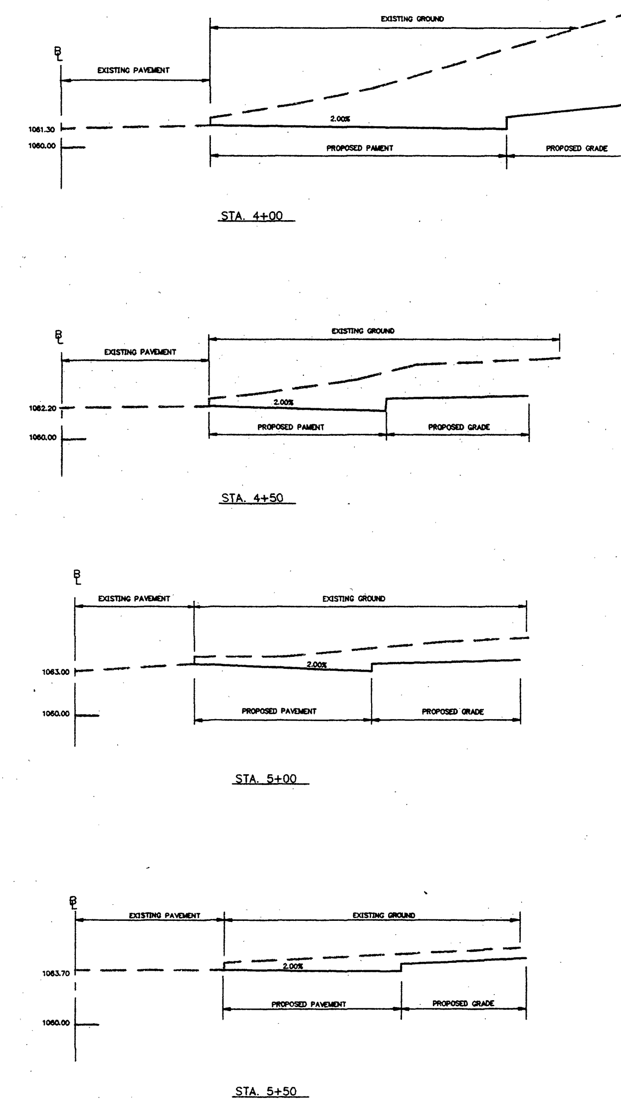
RING ROAD CROSS-SECTIONS SCALE 1"=5'
