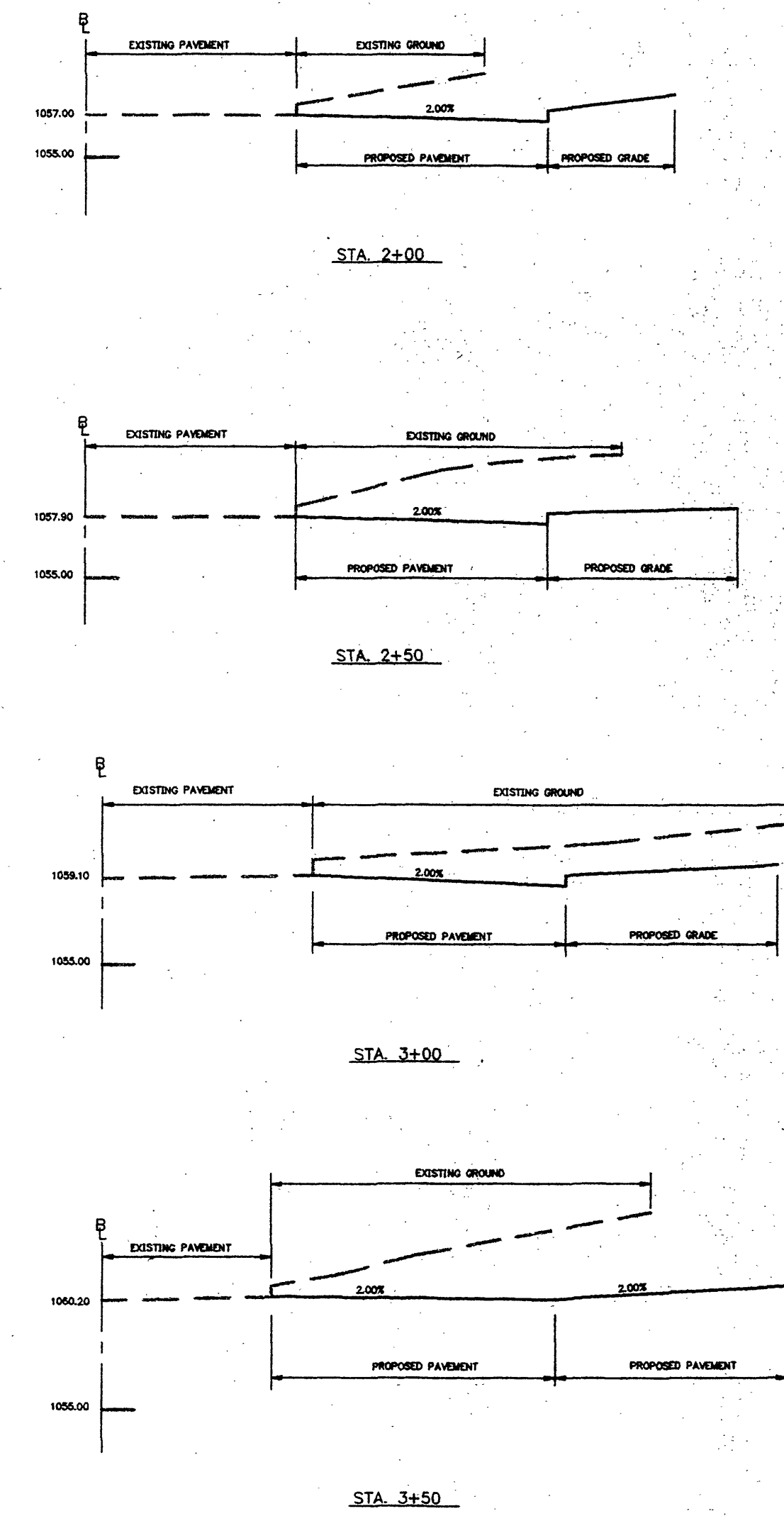
RING ROAD CROSS-SECTIONS SCALE 1"=5'
