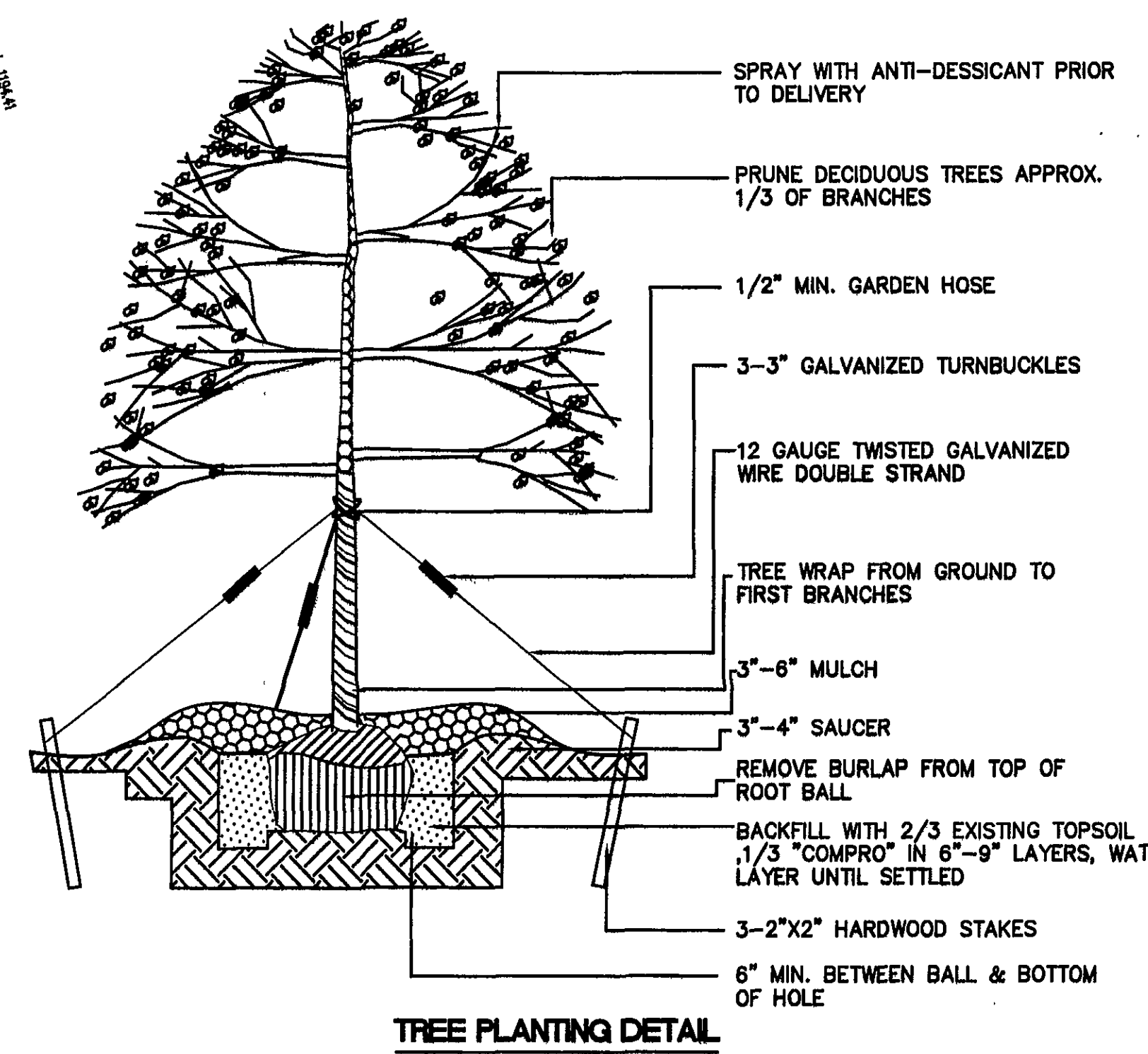
TREE PLANTING DETAIL
