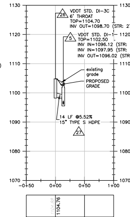
STR:26 TO STR:5 - STORM SEWER PROFILE
