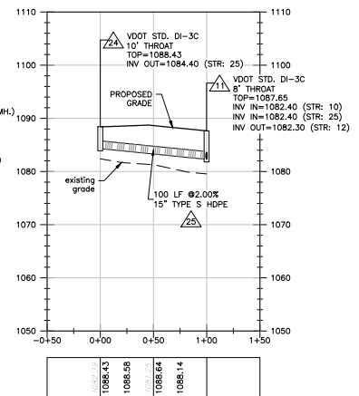
STR:24 TO STR:11 - STORM SEWER PROFILE
