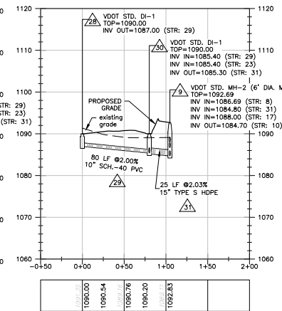
STR:28 TO STR:9 - STORM SEWER PROFILE
