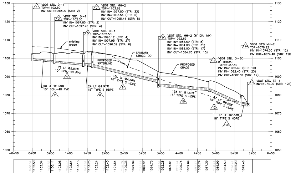
STR:1 TO STR:11 - STORM SEWER PROFILE
