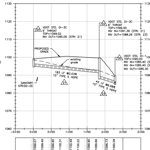
STR:20 TO STR:30 - STORM SEWER PROFILE
