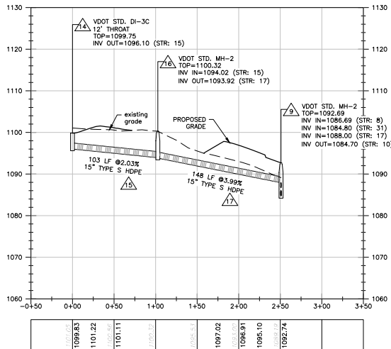
STR:14 TO STR:9 - STORM SEWER PROFILE
