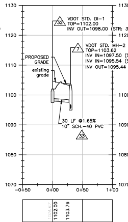
STR:32 TO STR:7 - STORM SEWER PROFILE
