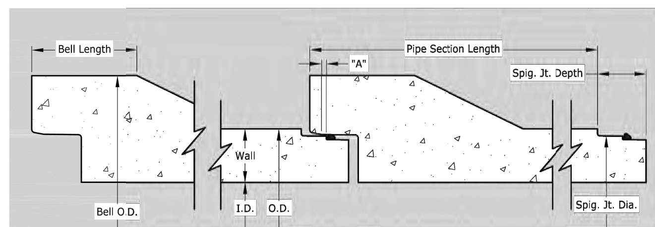
Section View
