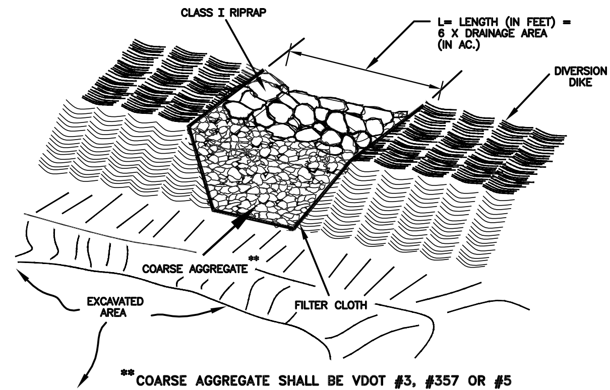
TEMPORARY SEDIMENT TRAP
