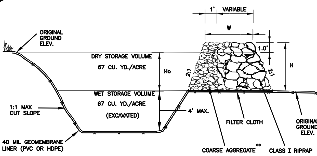
CROSS SECTION OF OUTLET
