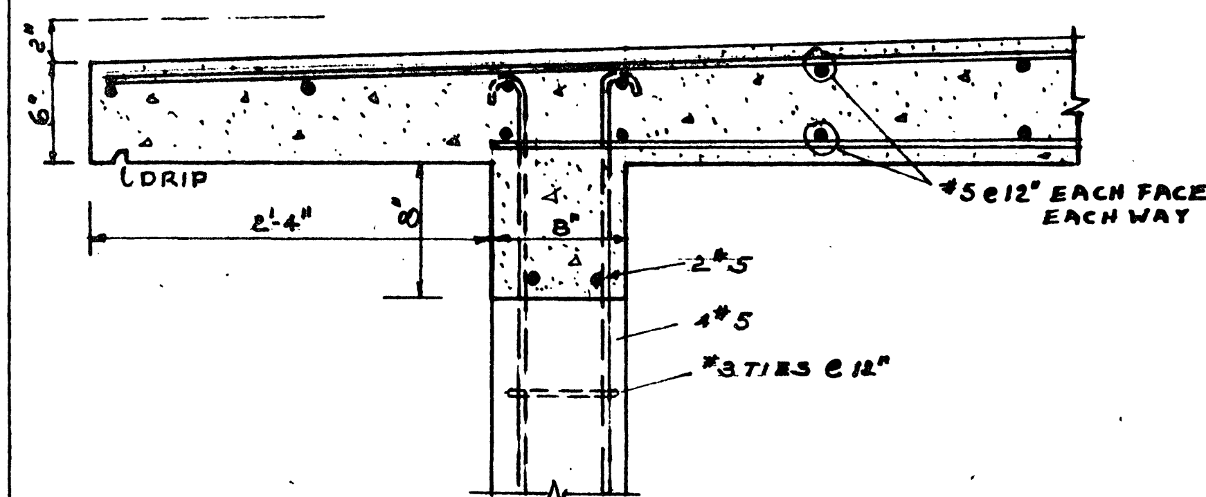
CONC. COLUMN & BEAM DETAIL SCALE 1/2" = 1'-0"
