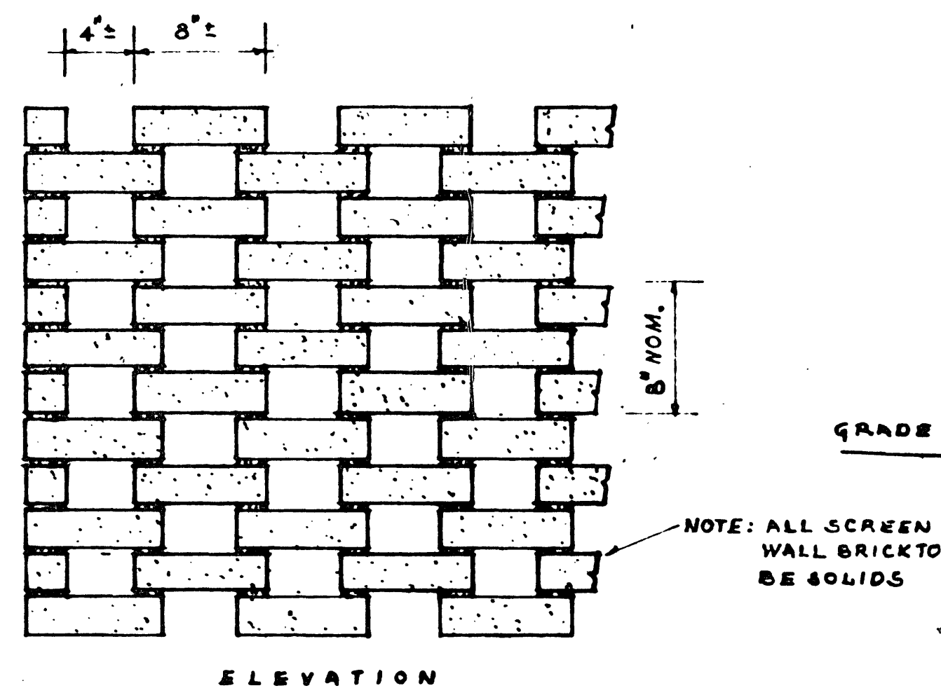
TYP. SCREEN WALL DETAIL SCALE 1/2" = 1'-0"
