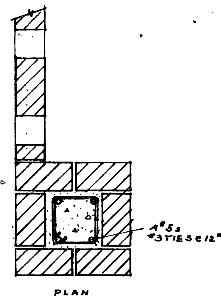
CORNER COLUMN DETAIL SCALE 1/2" = 1'-0"
