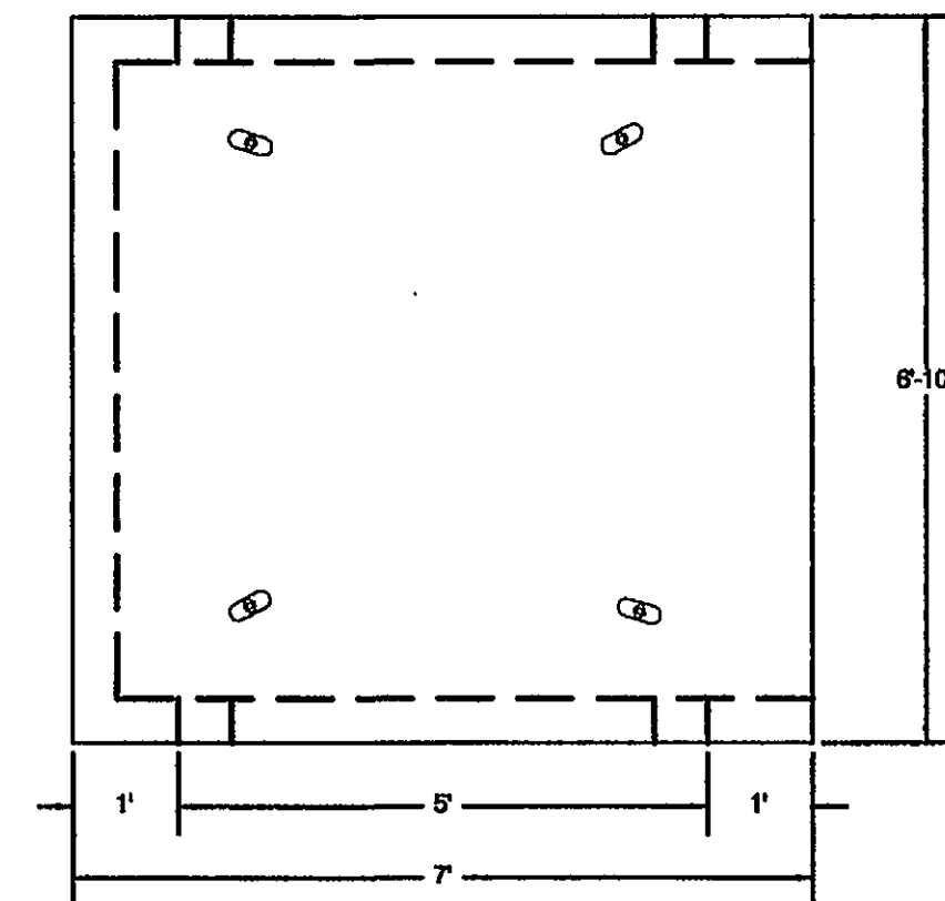
PLAN VIEW
