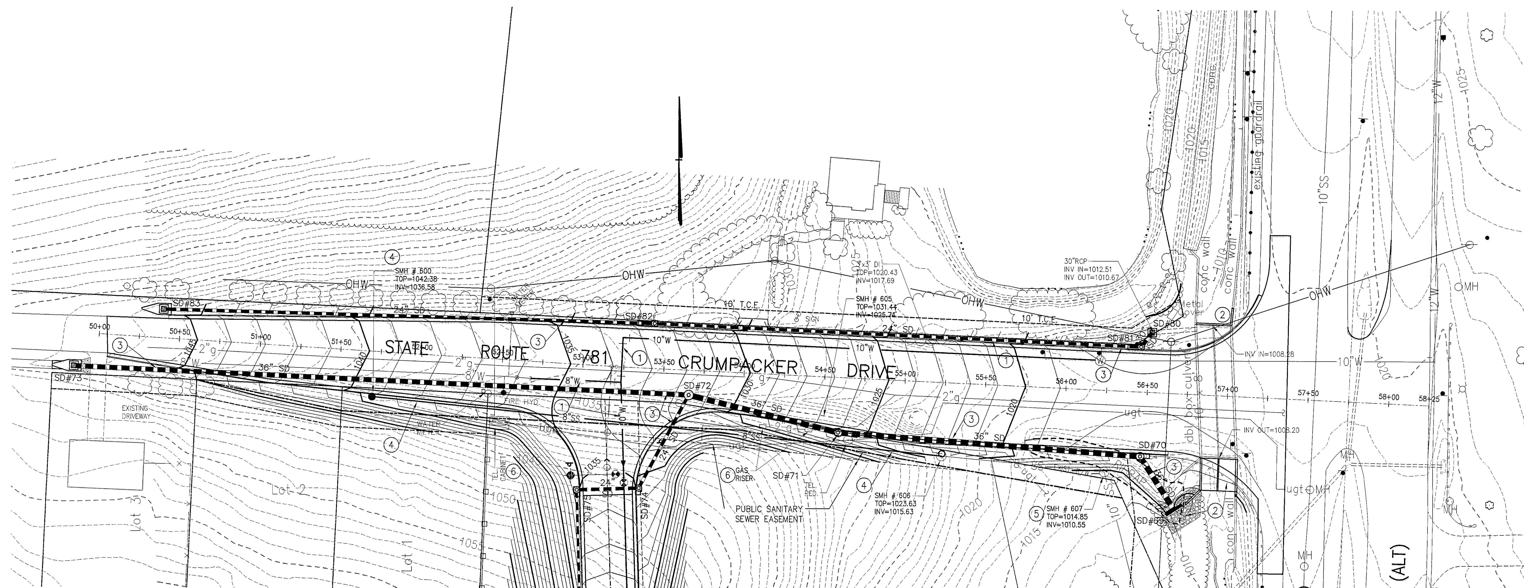
GRADING & UTILITY PLAN - CRUMPACKER DRIVE (RTE. 781)
