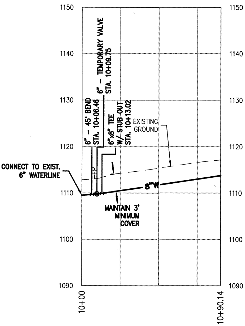
6 INCH & 8 INCH WATERLINE – MONROE ST.
