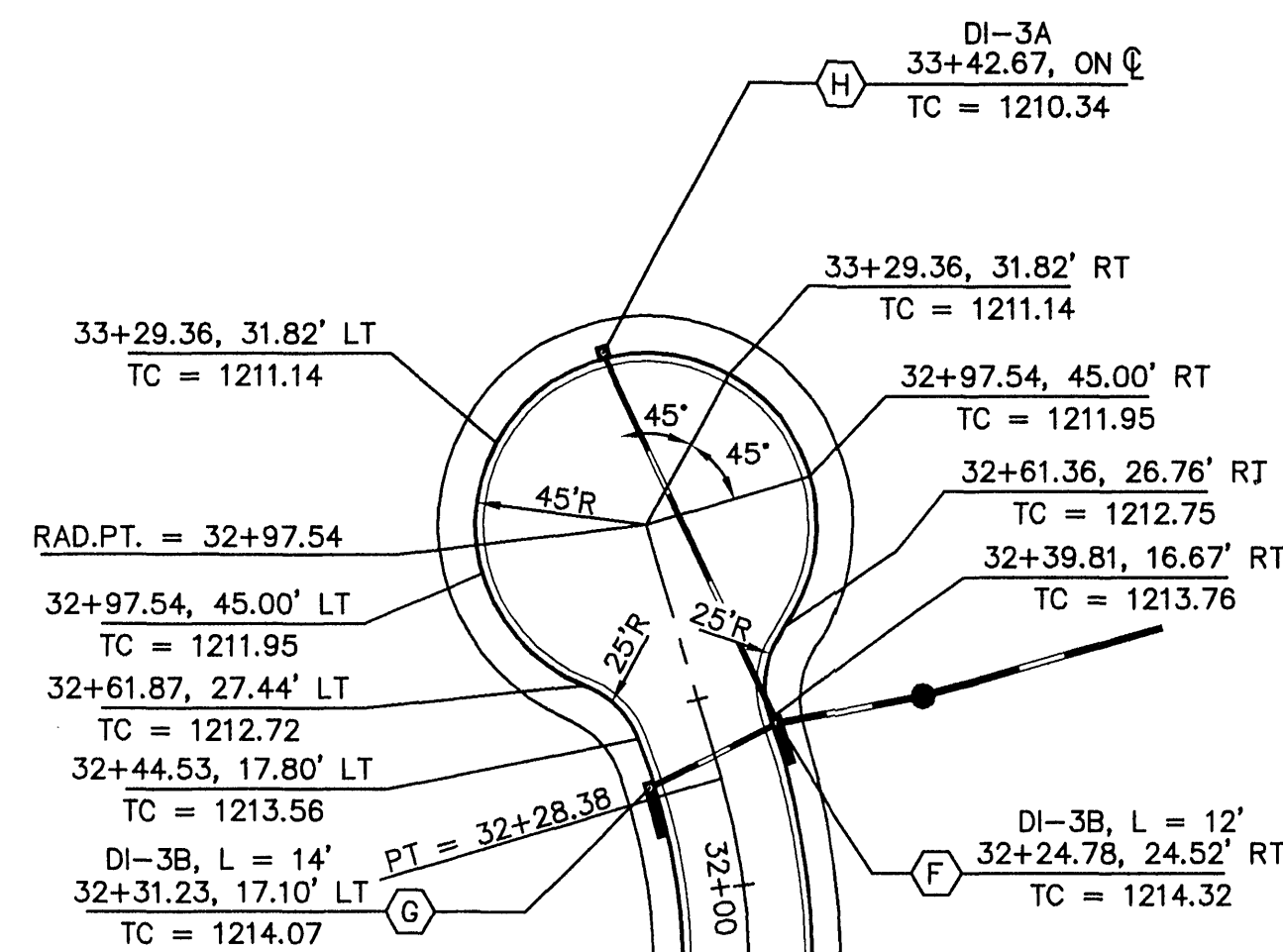
CUL-DE-SAC DETAIL
