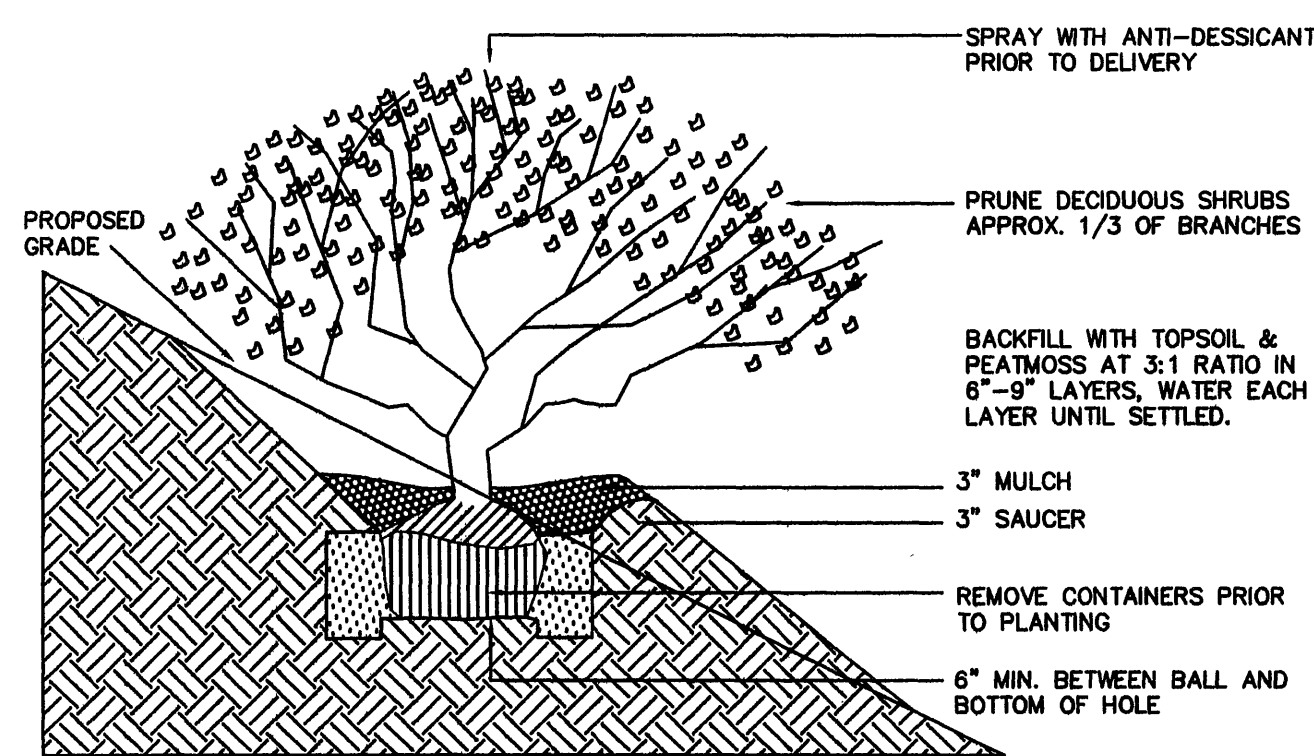
SLOPE PLANTING DETAIL NOT TO SCALE
