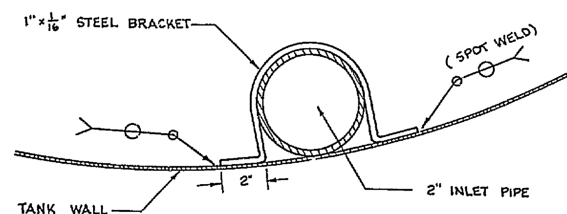
PIPE SUPPORT BRACKET DETAIL NOT TO SCALE
