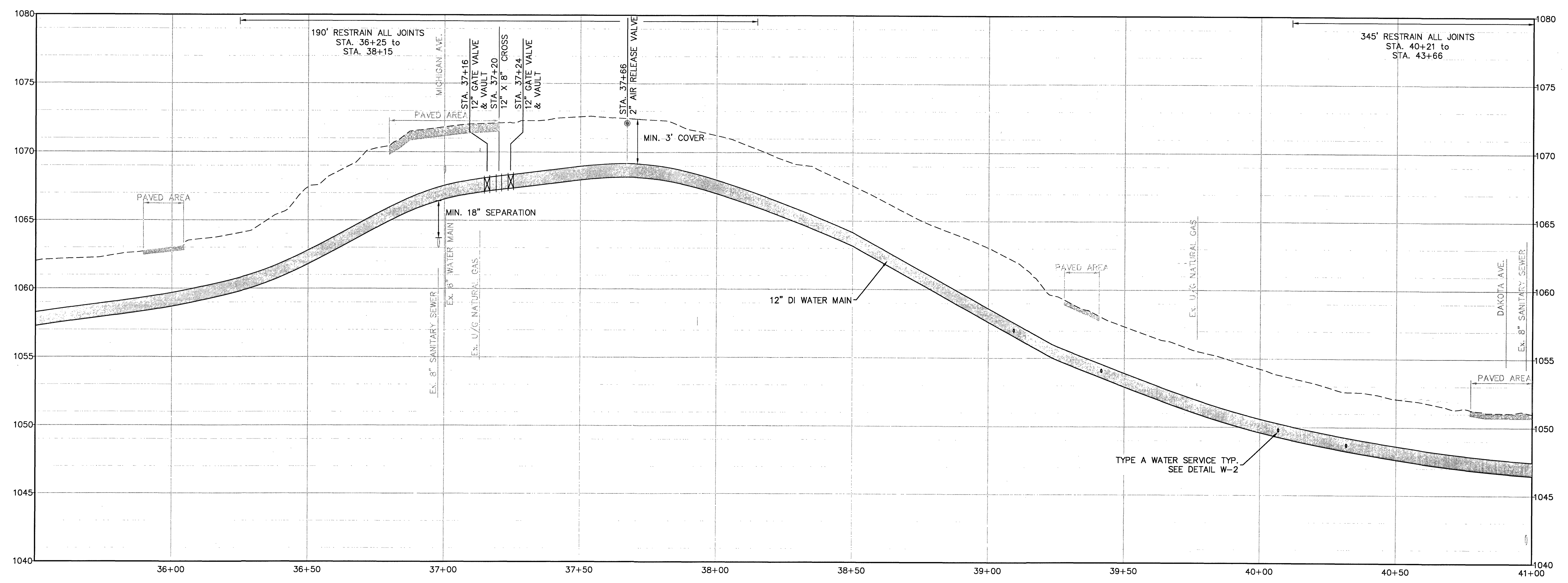
WATER MAIN PROFILE SCALE: H:1"=20' V:1"=4'
