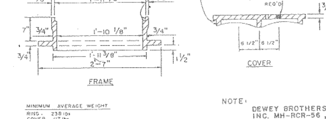
MANHOLE FRAME AND COVER
