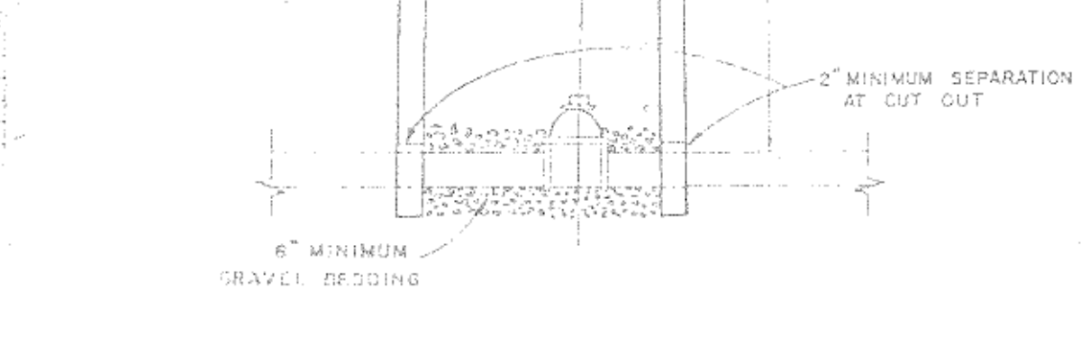
ALTERNATE VALVE VAULT (MANHOLE)
