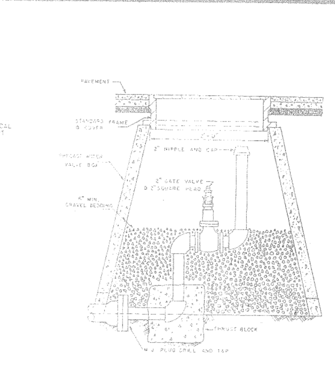
PERMANENT END OF LINE
