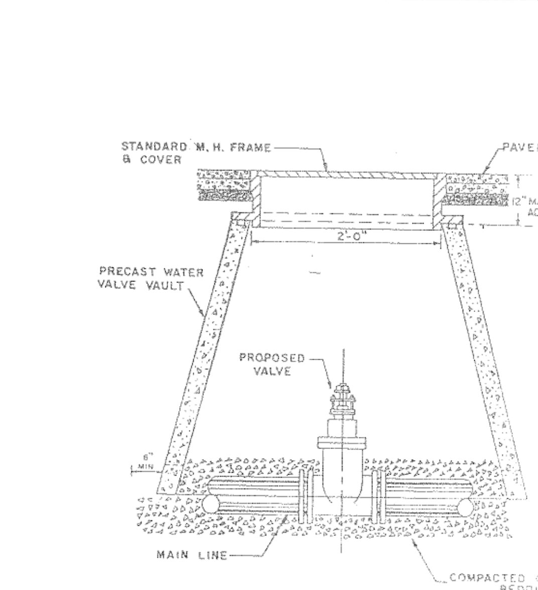
WATER LINE VALVE INSTALLATION
