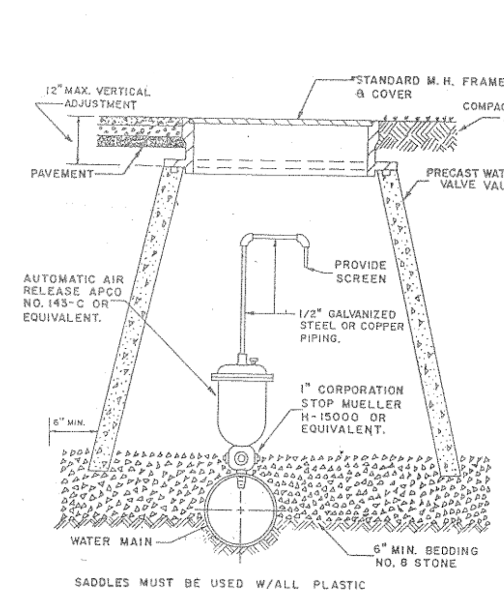
AUTOMATIC AIR RELEASE ASSEMBLY
