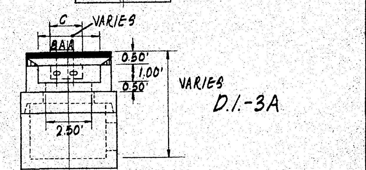
THROAT PLATE LOCATIONS ON CURB INLETS NO SCALE
