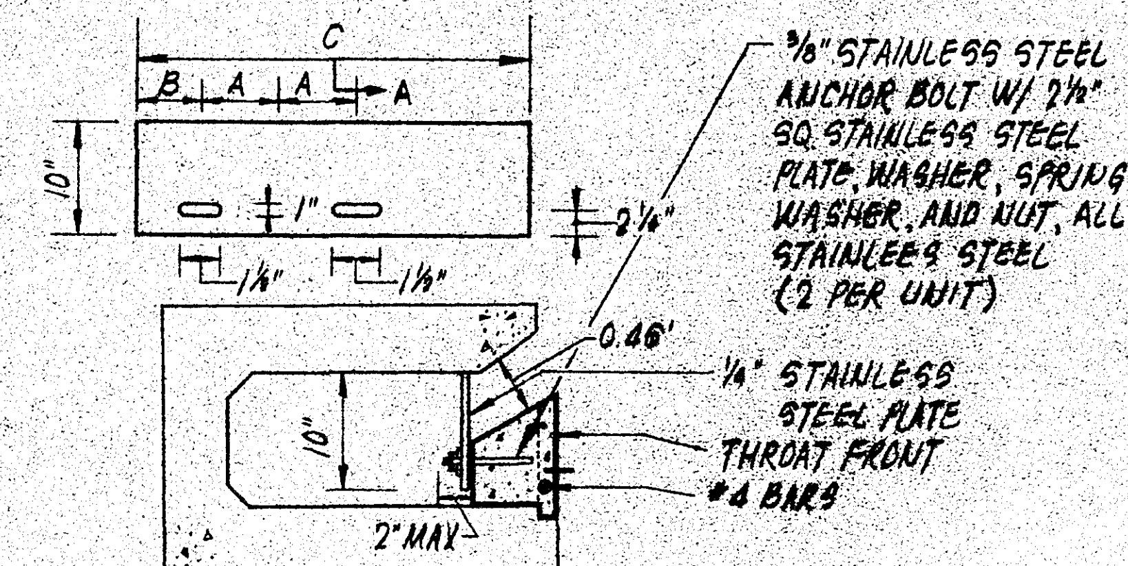
SECTION A-A INLET THROAT PLATES
