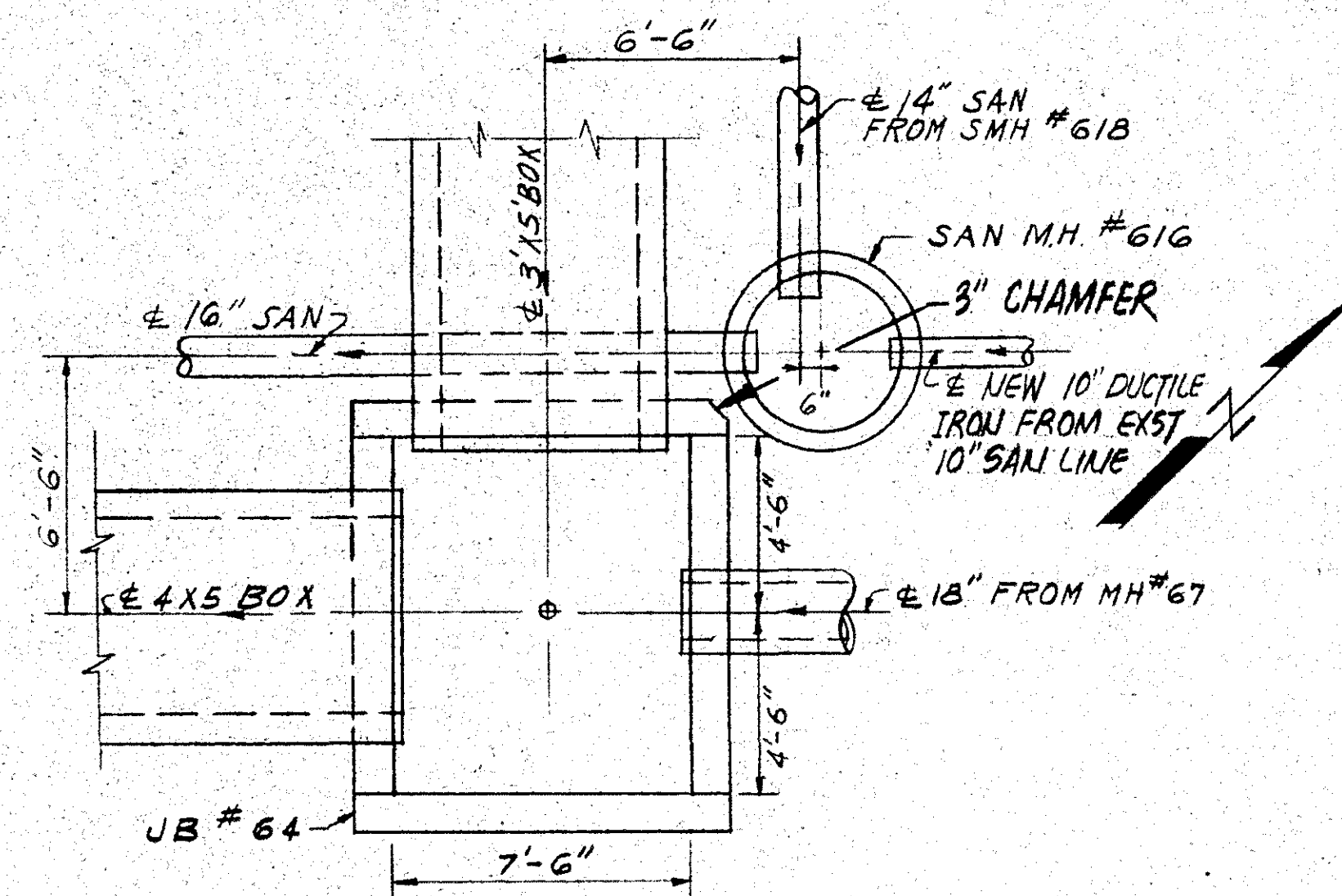
SANITARY MANHOLE #616
