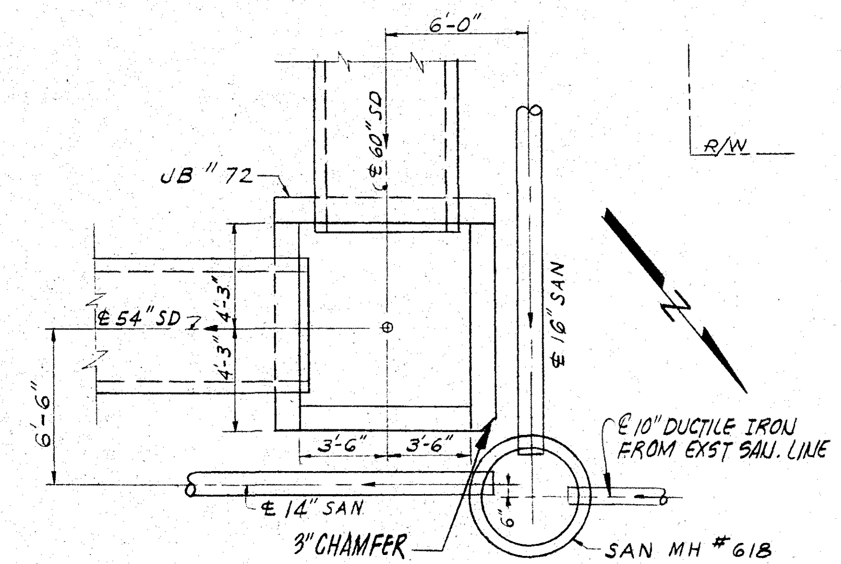
SANITARY MANHOLE #618
