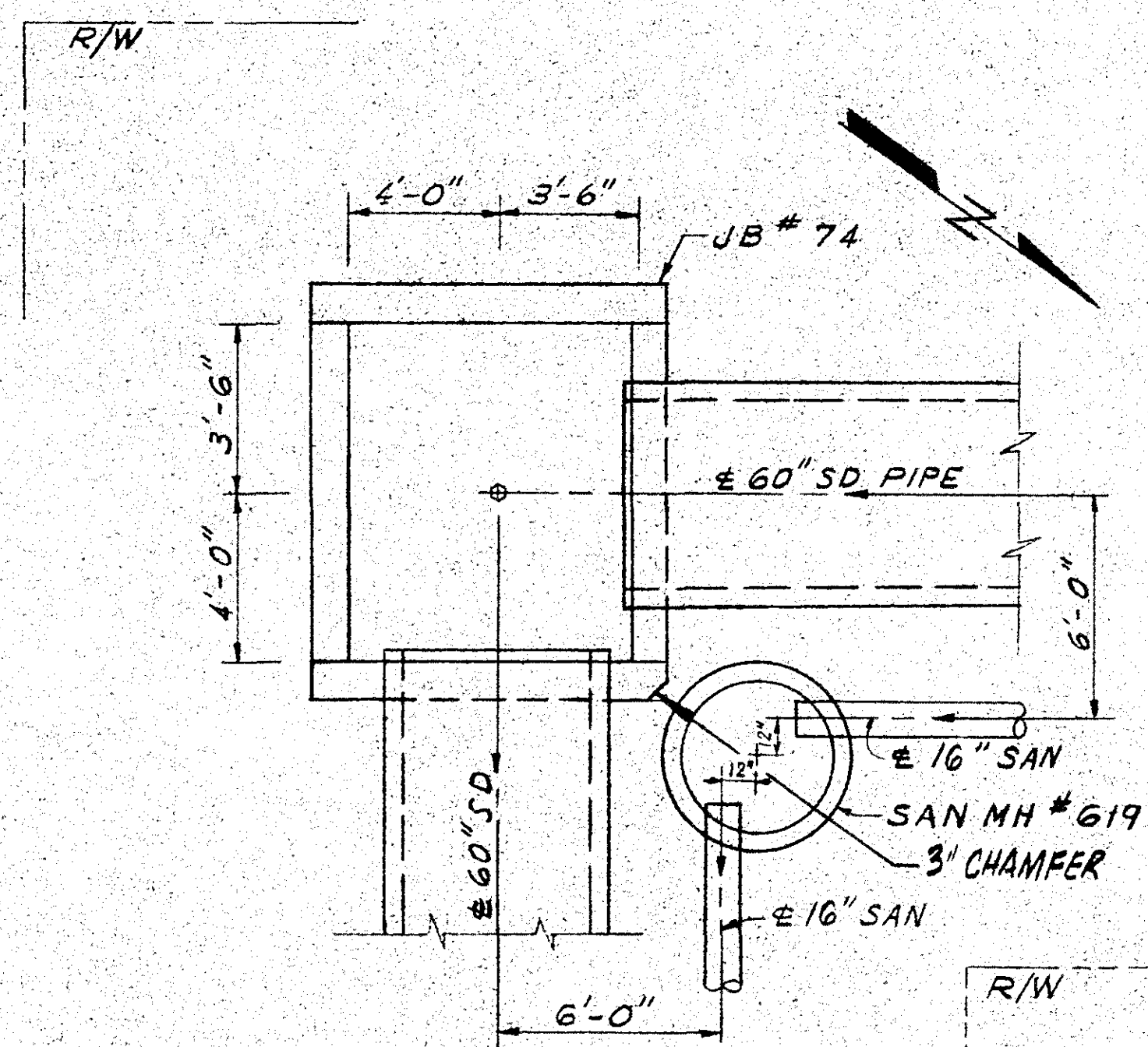
SANITARY MANHOLE #619
