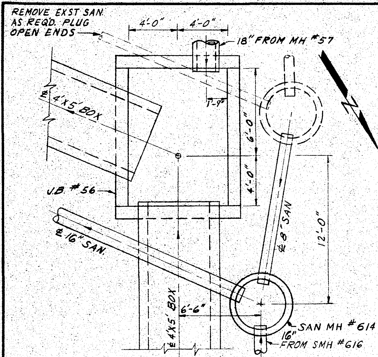
SANITARY MANHOLE #614
