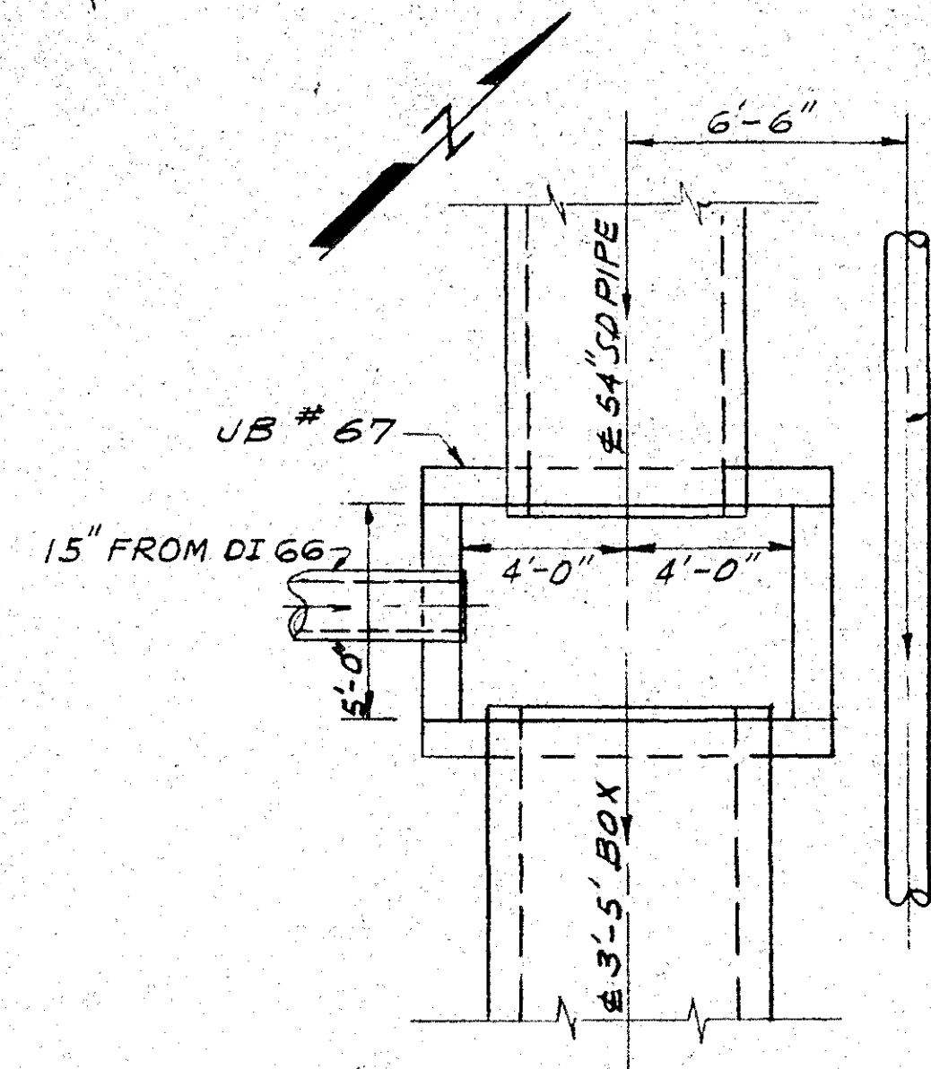
SANITARY SEWER LINE
