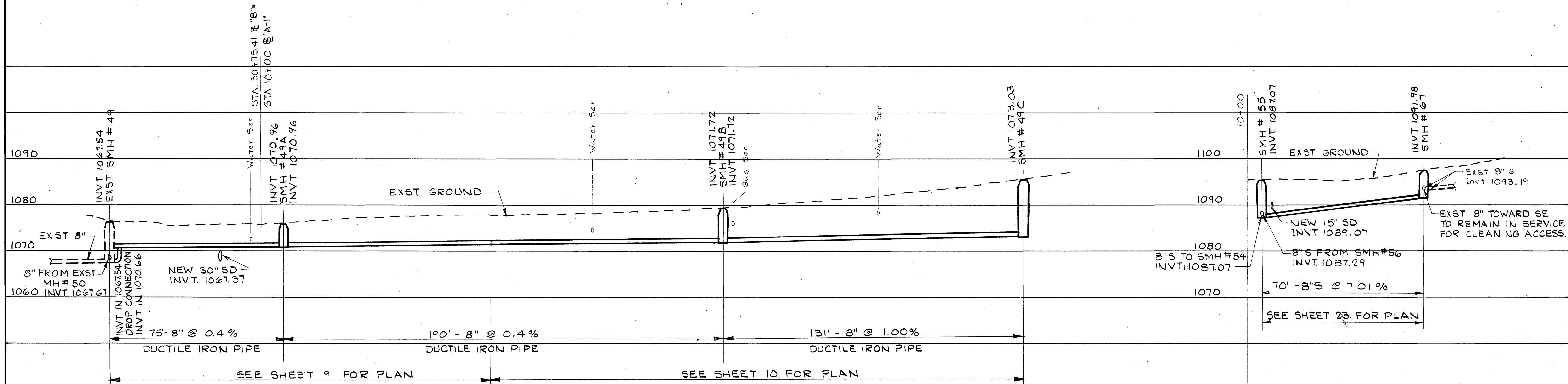
PROFILE - 8" SANITARY - RAVENWOOD AVE. (N.I.C.)
