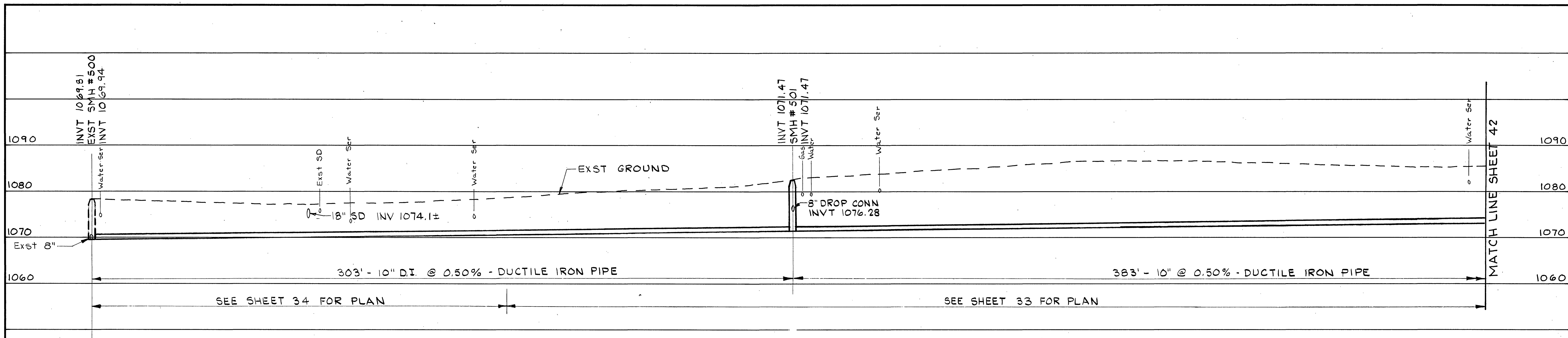
PROFILE-10" SANITARY - FLORALAND DRIVE
