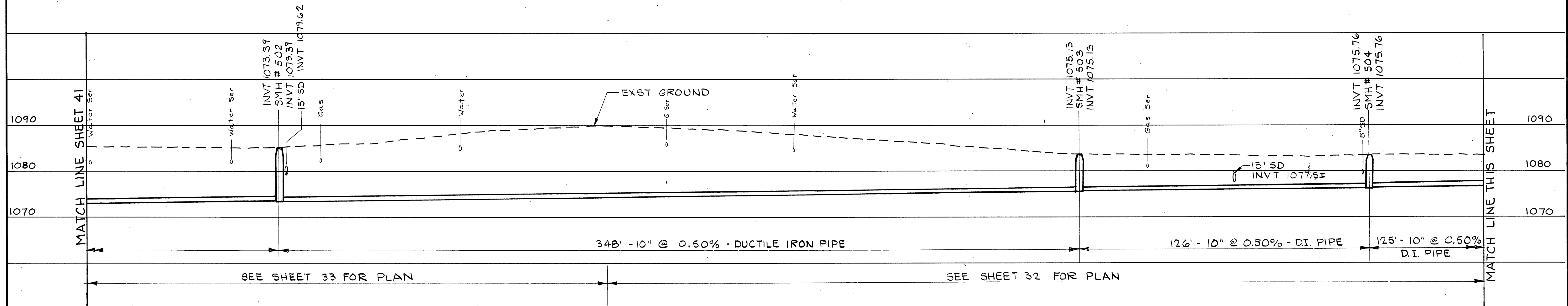
PROFILE - 10" SANITARY - FLORALAND DRIVE
