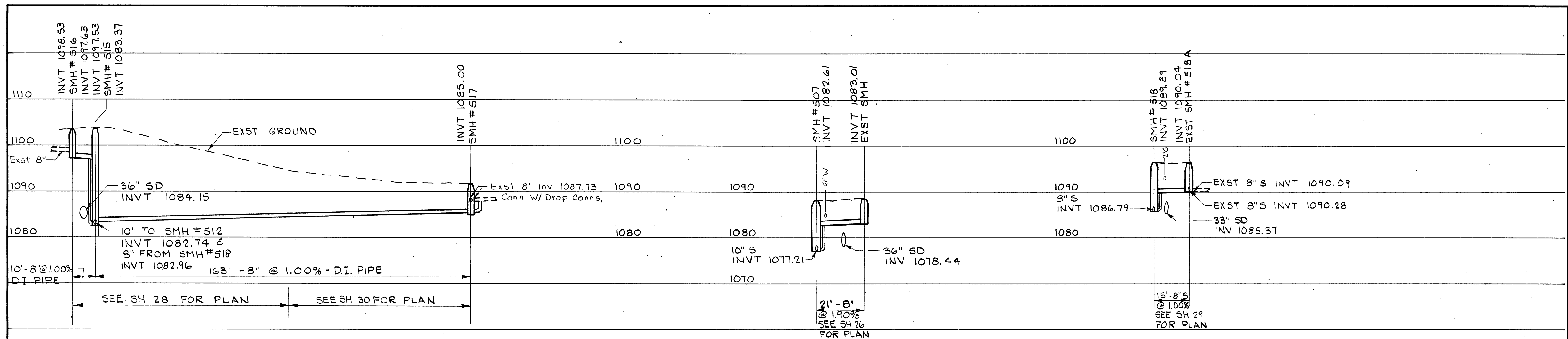
PROFILE - 8" SANITARY - CORNELL DR
