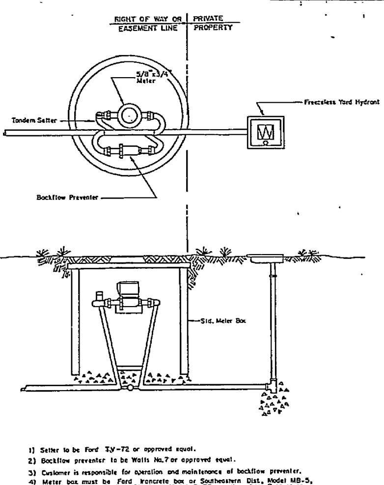
TYPICAL SPRINKLER SERVICE
