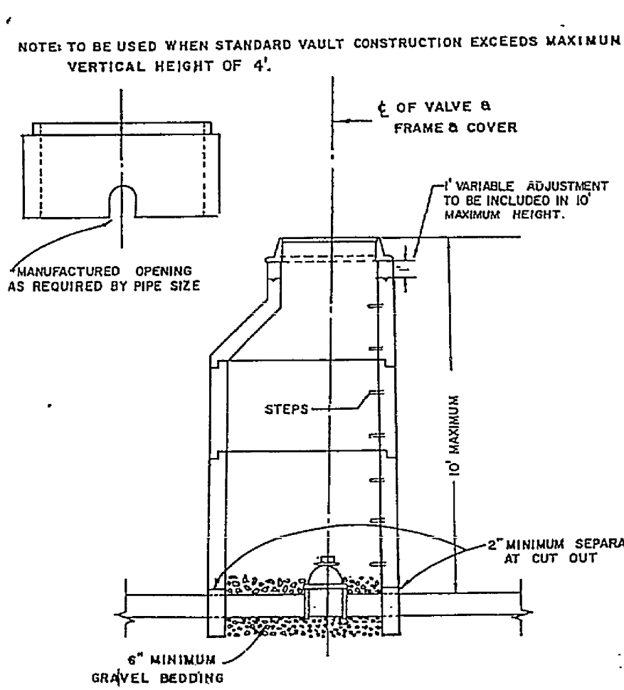
ALTERNATE VALVE VAULT (MANHOLE)
