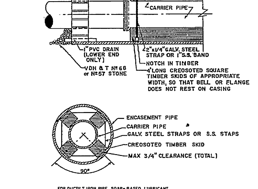
PIPE SUPPORT IN CASING PIPE
