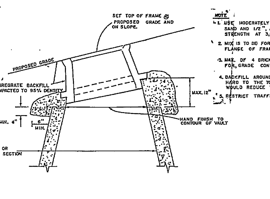
MANHOLE FRAME & COVER ADJUSTMENT
