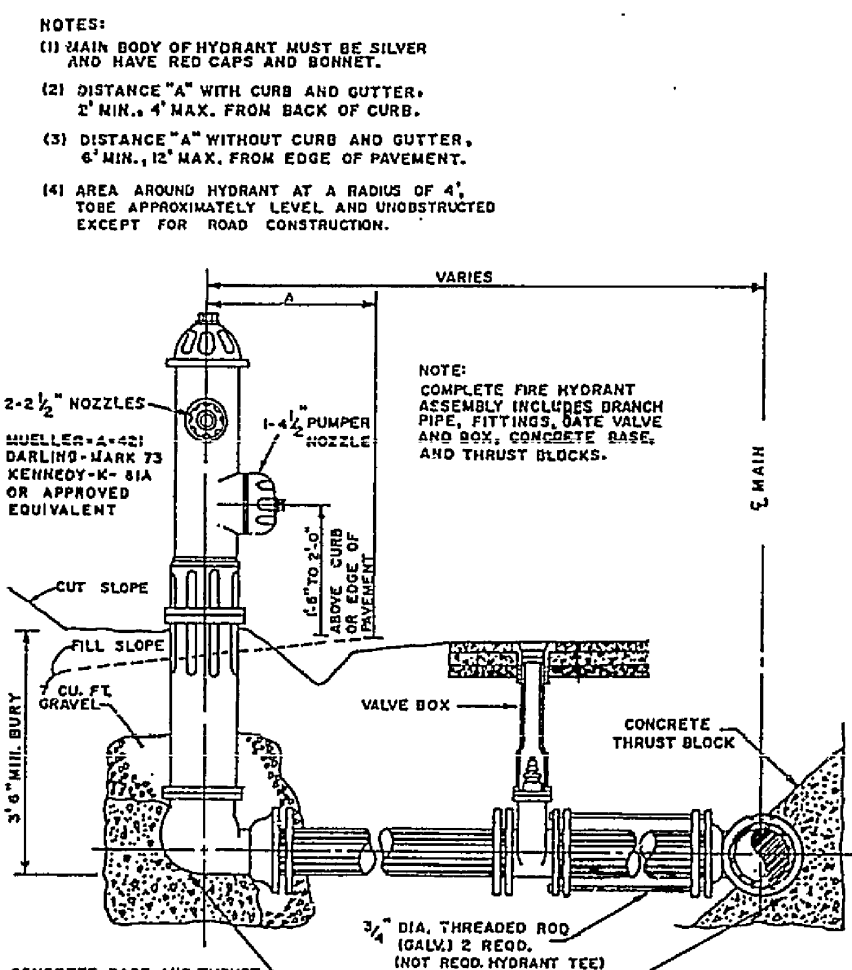
FIRE HYDRANT SETTING
