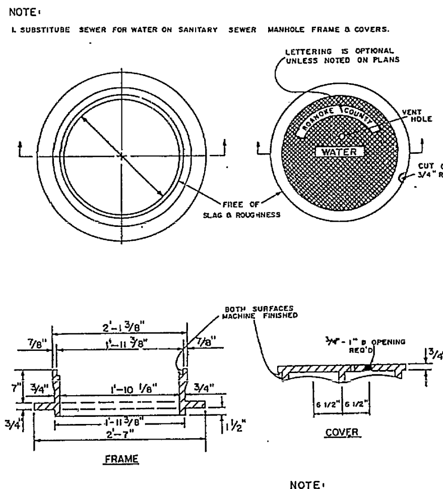
MANHOLE FRAME AND COVER
