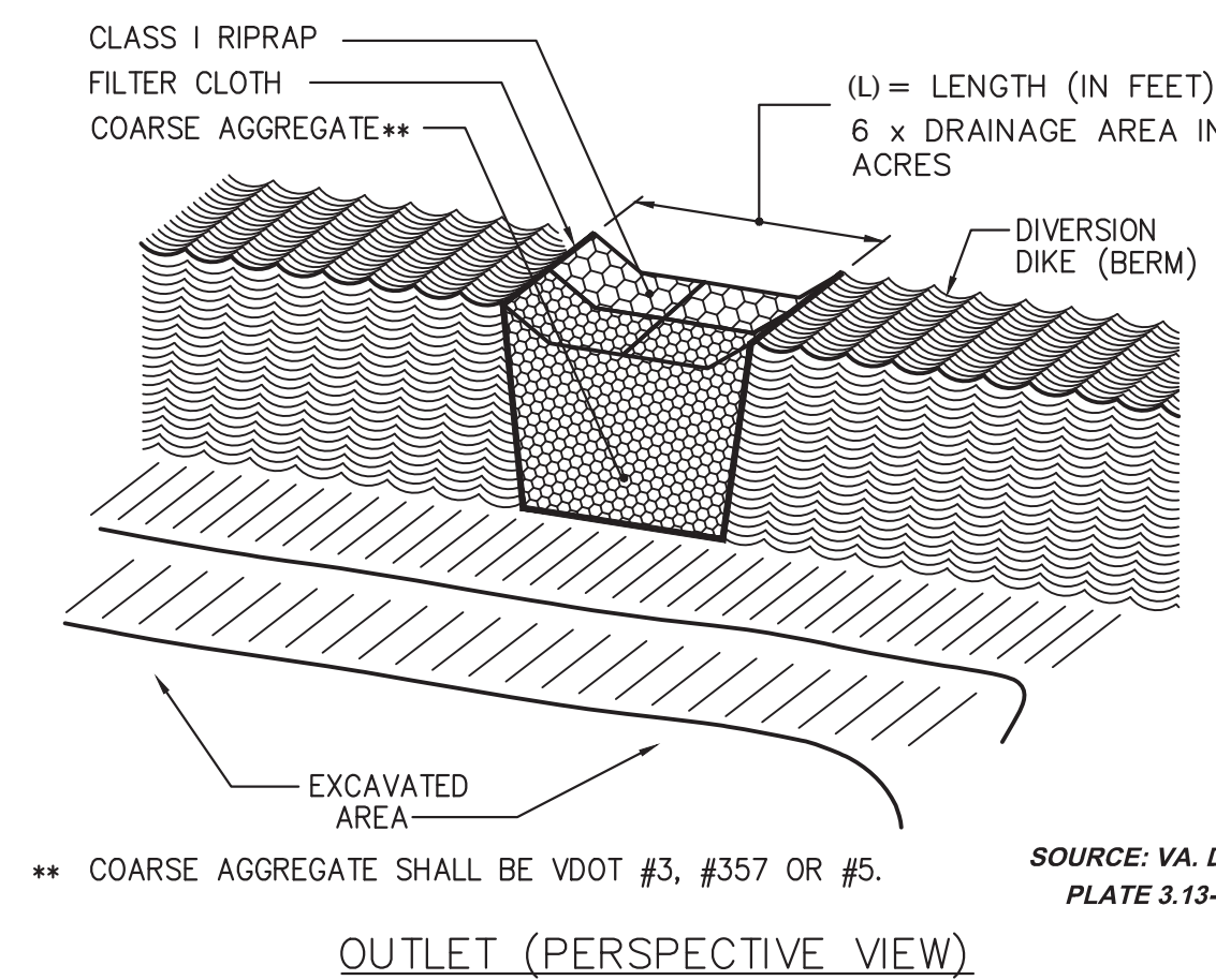
3.13A TEMPORARY SEDIMENT TRAP C400 C801 NOT TO SCALE
