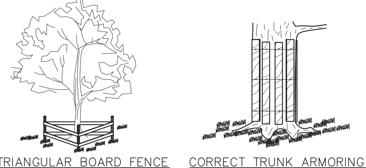
3.38 TREE PROTECTION – FENCING AND ARMORING C400/C801 NOT TO SCALE
