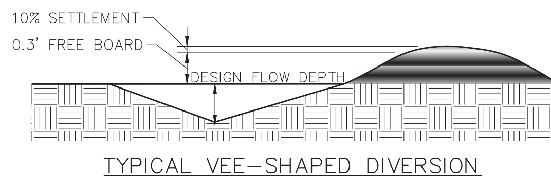
3.12 TYPICAL DIVERSIONS C400 | C801 NOT TO SCALE
