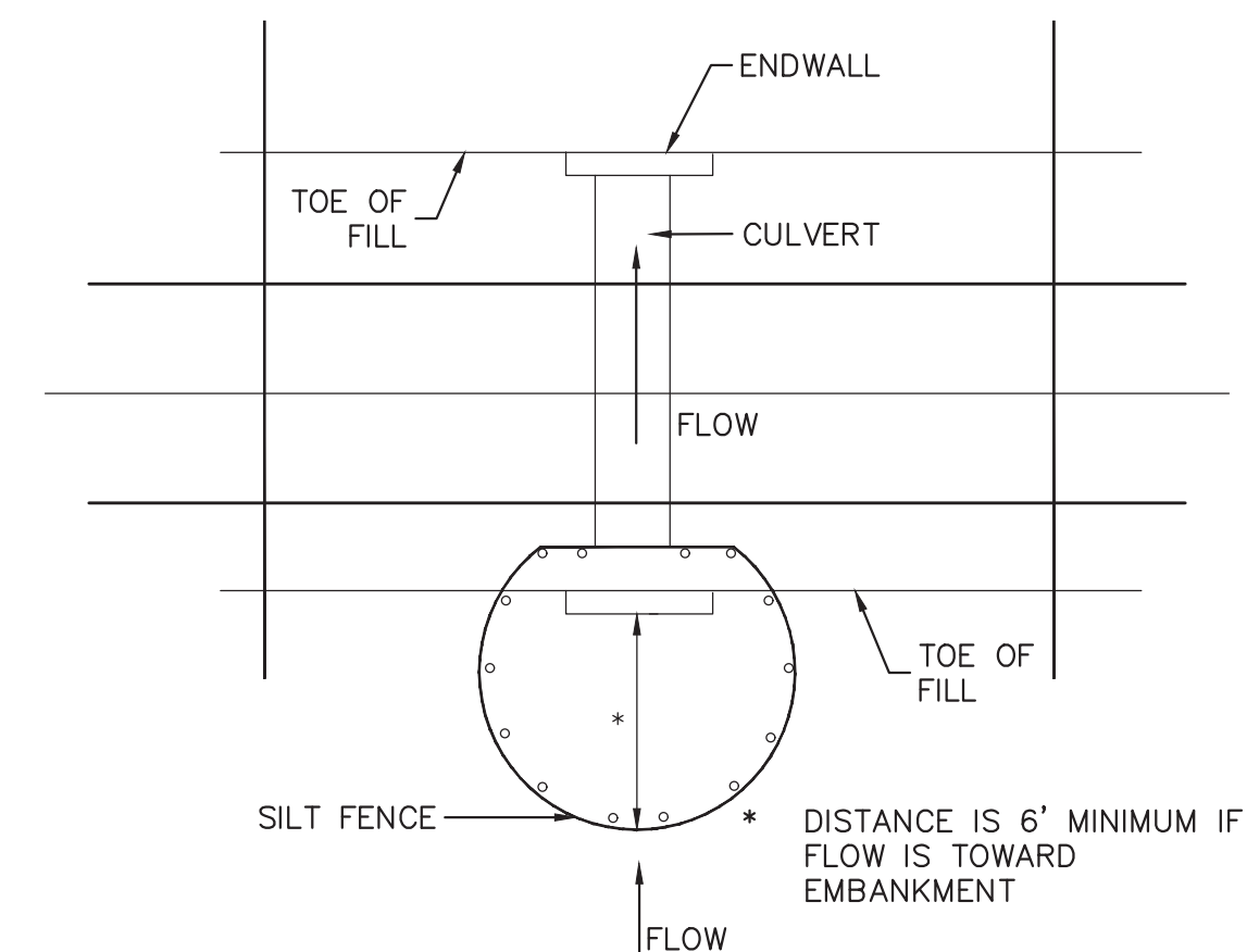
3.13B TEMPORARY SEDIMENT TRAP CALCULATIONS C400 C801 NOT TO SCALE
