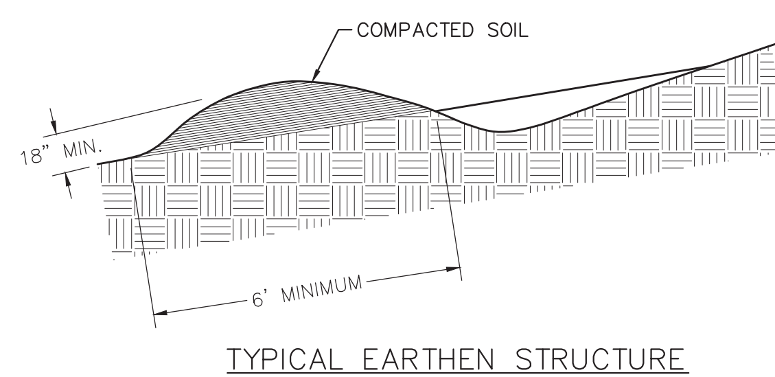
C400 C801 TEMPORARY RIGHT-OF-WAY DIVERSIONS NOT TO SCALE
