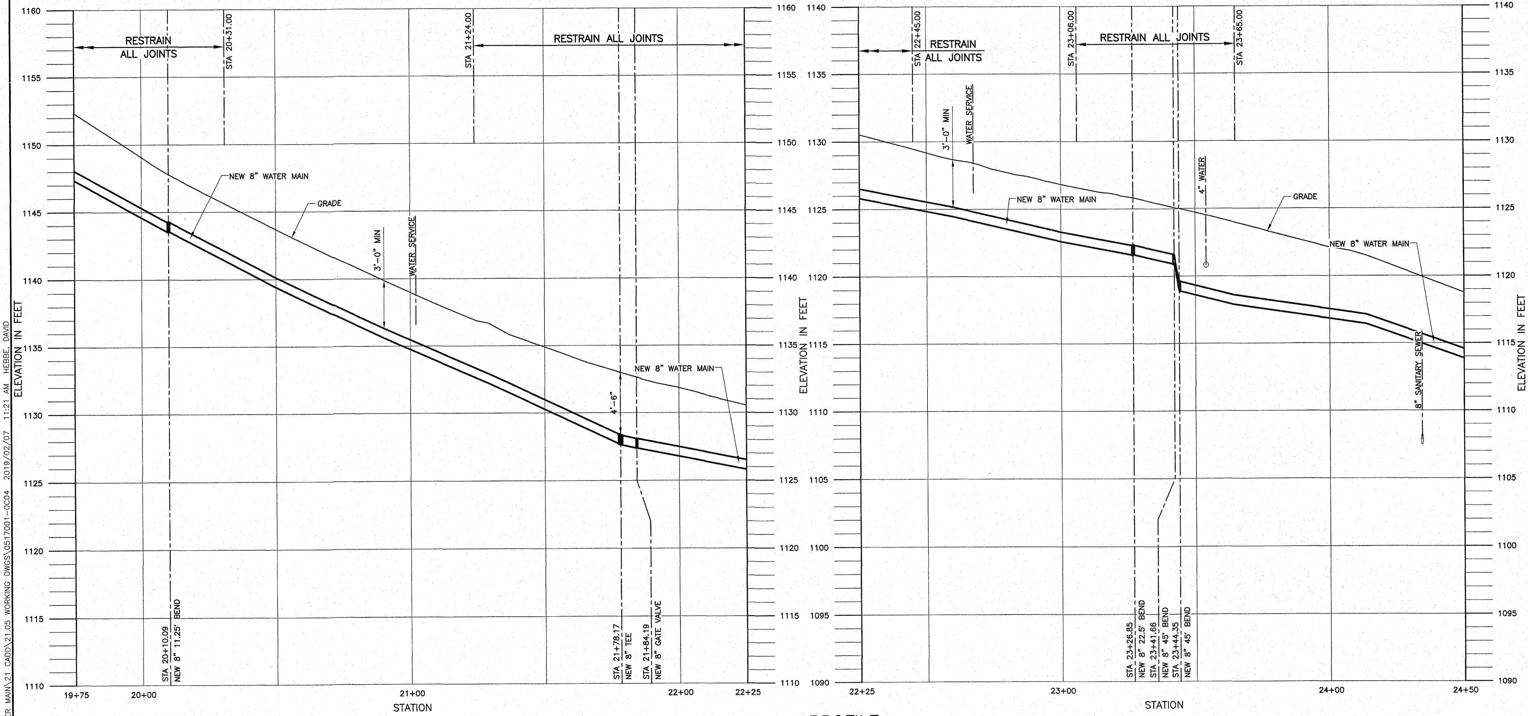
PROFILE SCALE: HORIZONTAL 1" = 20' VERTICAL 1" = 4'
