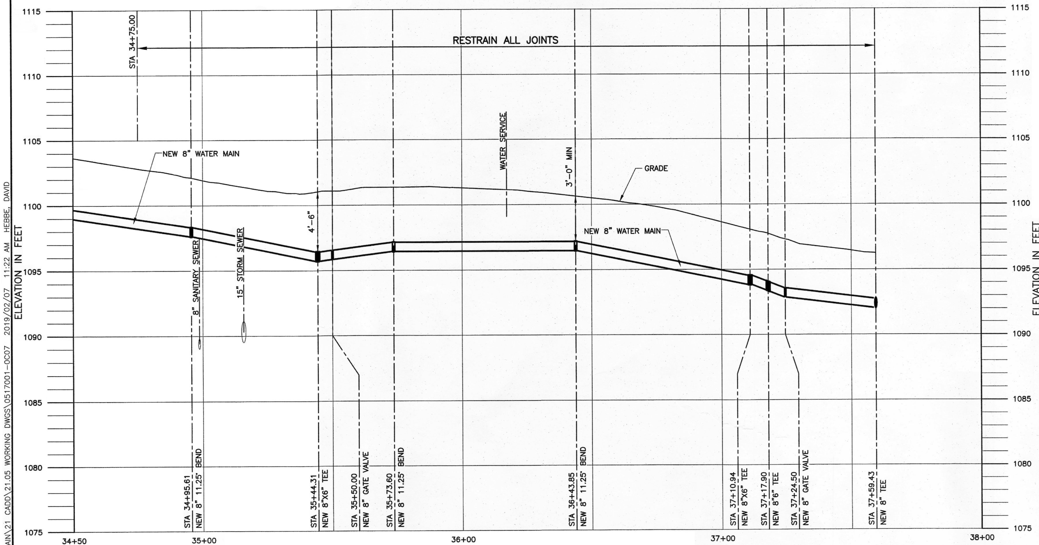
PROFILE SCALE: HORIZONTAL 1" = 20' VERTICAL 1" = 4'
