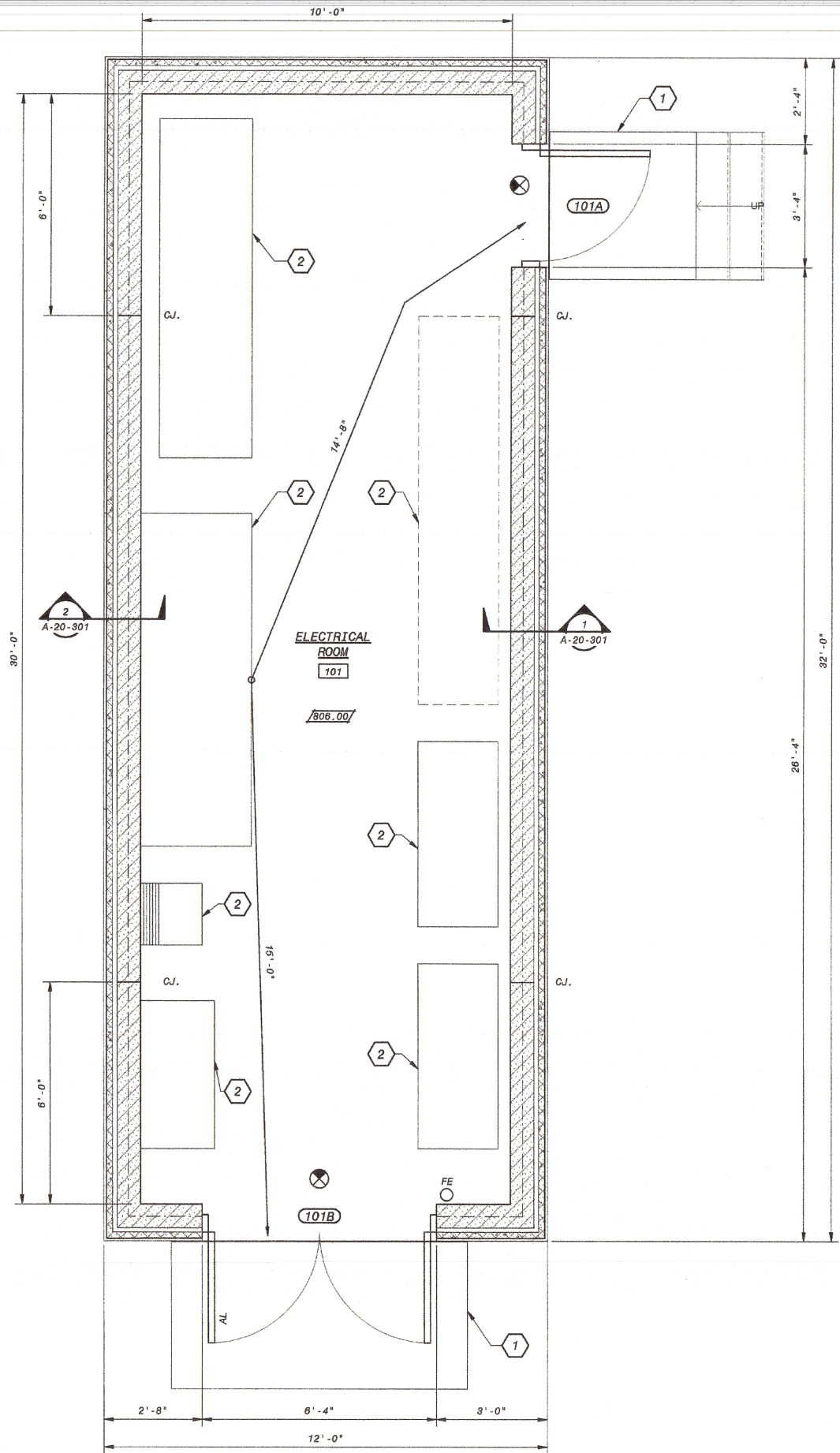
OPERATING FLOOR/LIFE SAFETY PLAN 1/2" = 1'-0"
