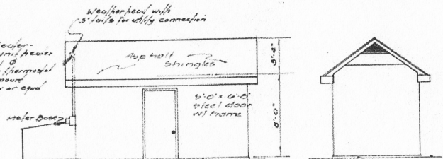
FRONT ELEVATION RIGHT SIDE
