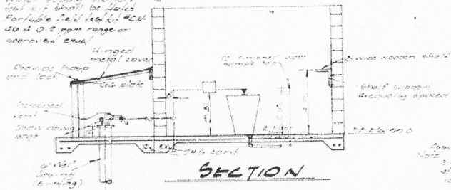
WELL HOUSE DETAIL
