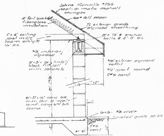
TYPICAL WALL SECTION
