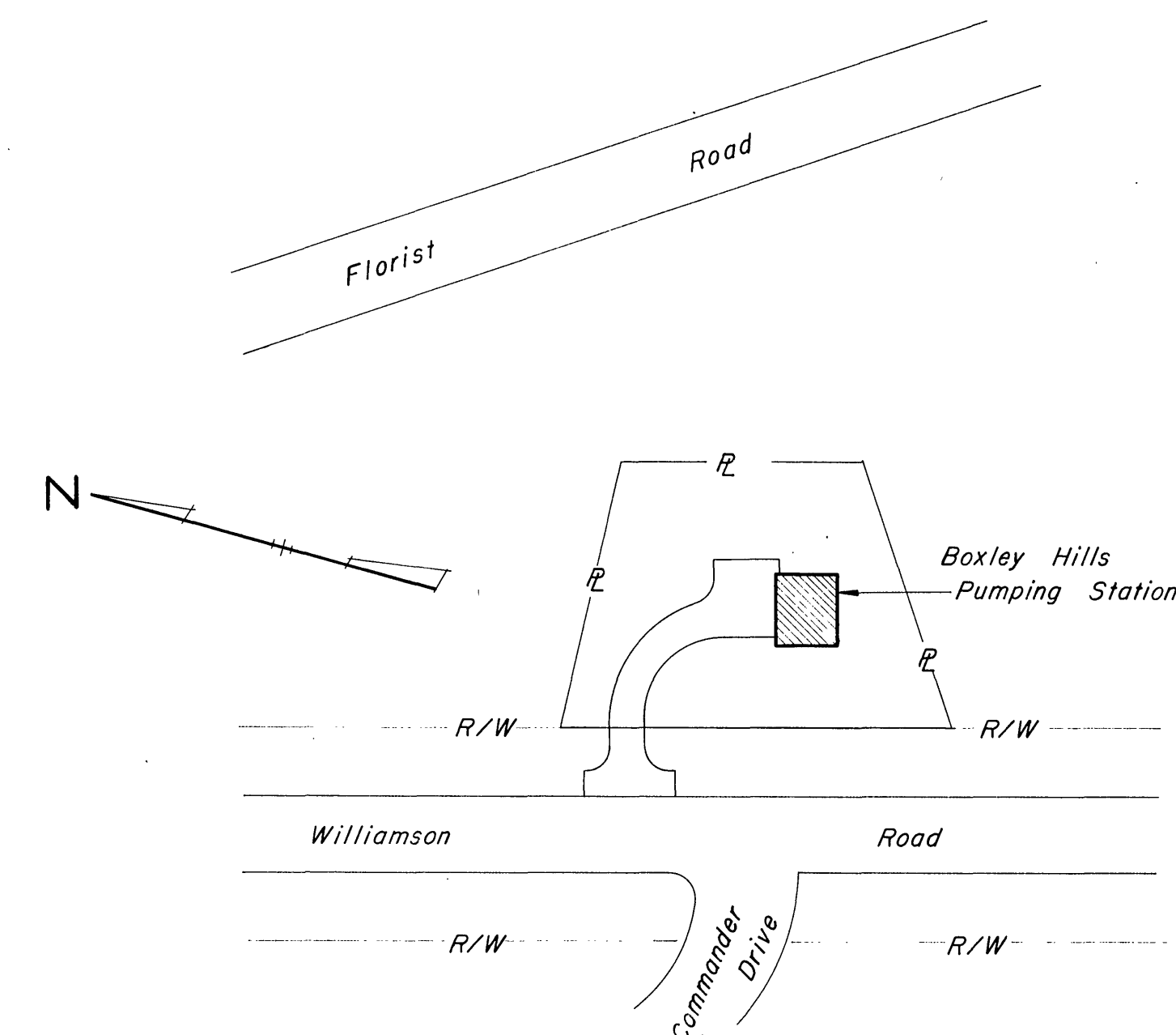
LOCATION PLAN SCALE: 1" = 60'
