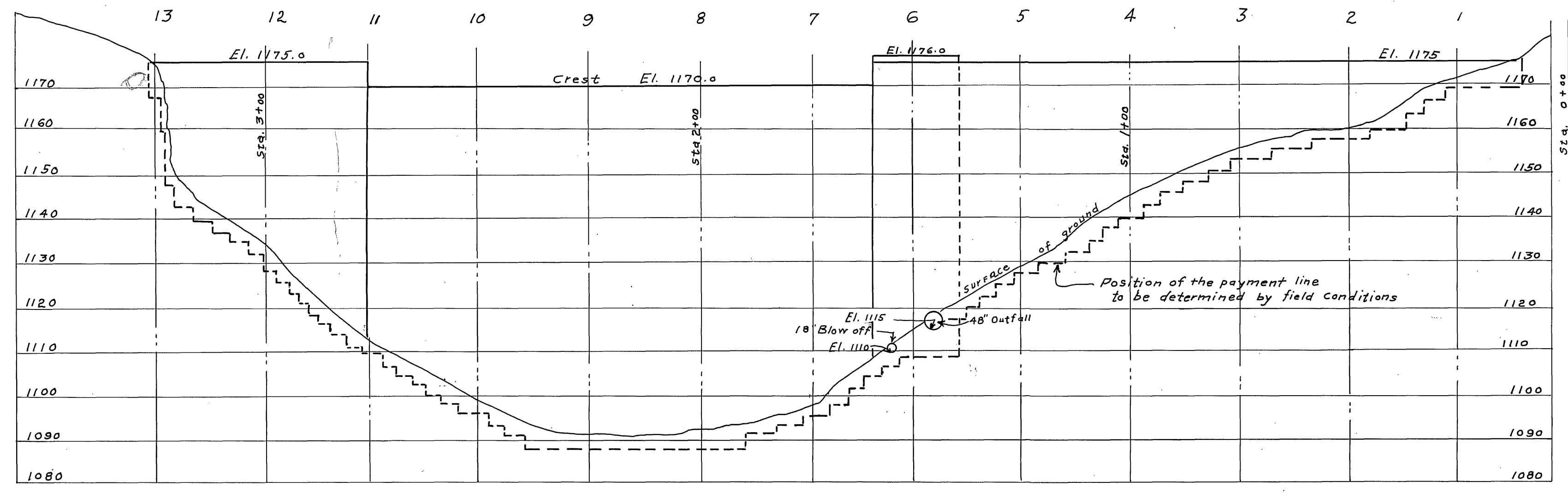
PROFILE OF DAM ON CENTER LINE
