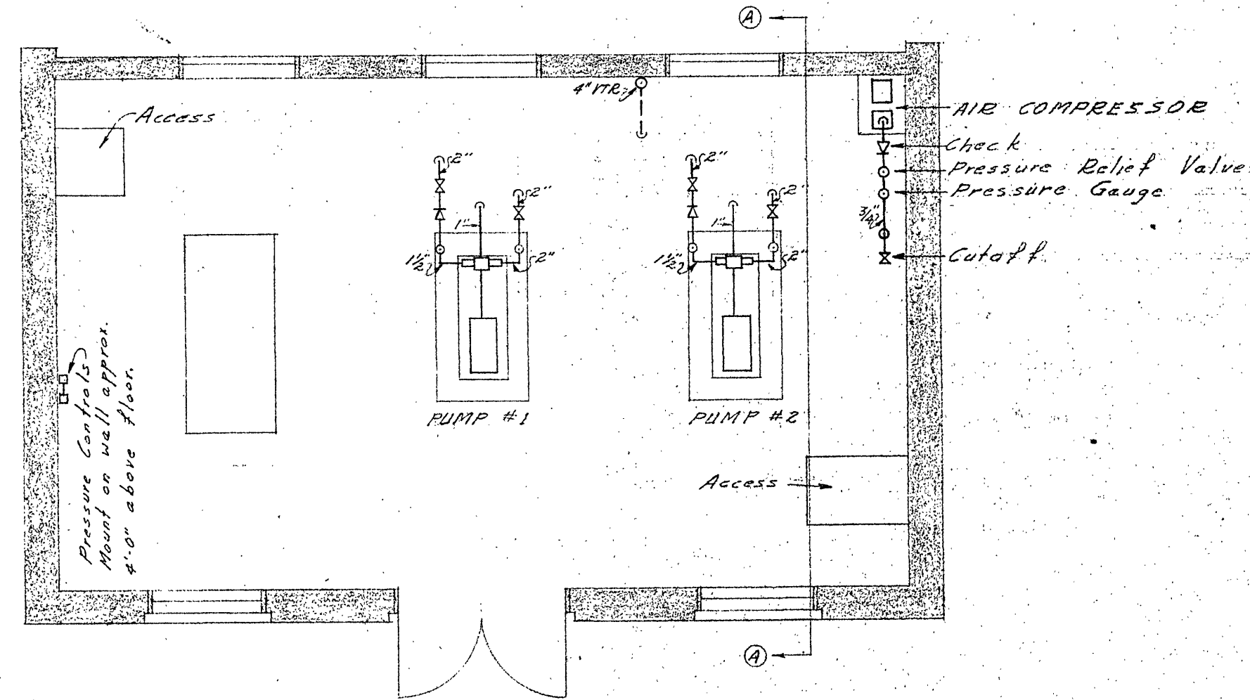
PLAN OF PUMP ROOM SCALE: 1/4" = 1'-0"
