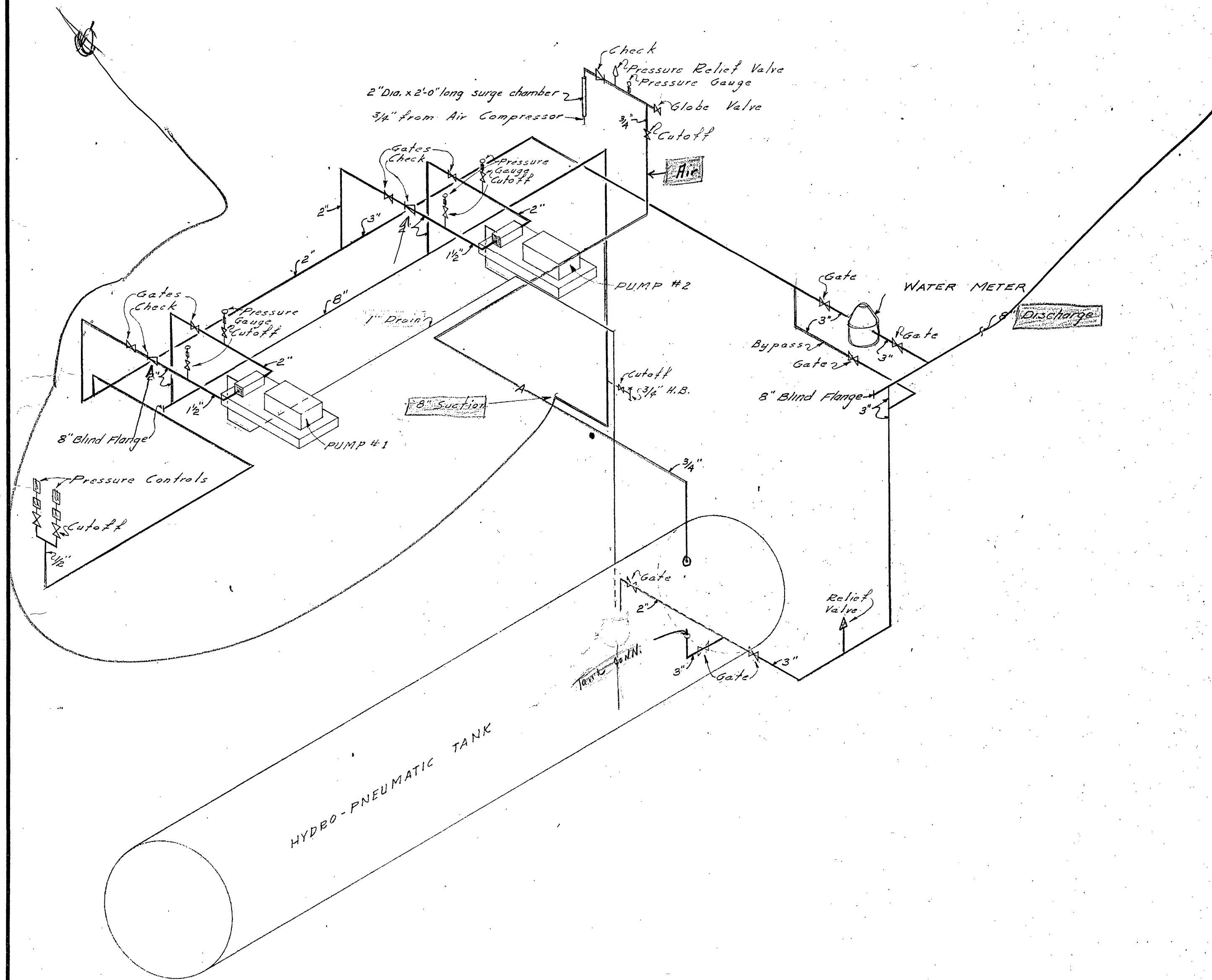
ISOMETRIC DETAIL OF PIPING NO SCALE
