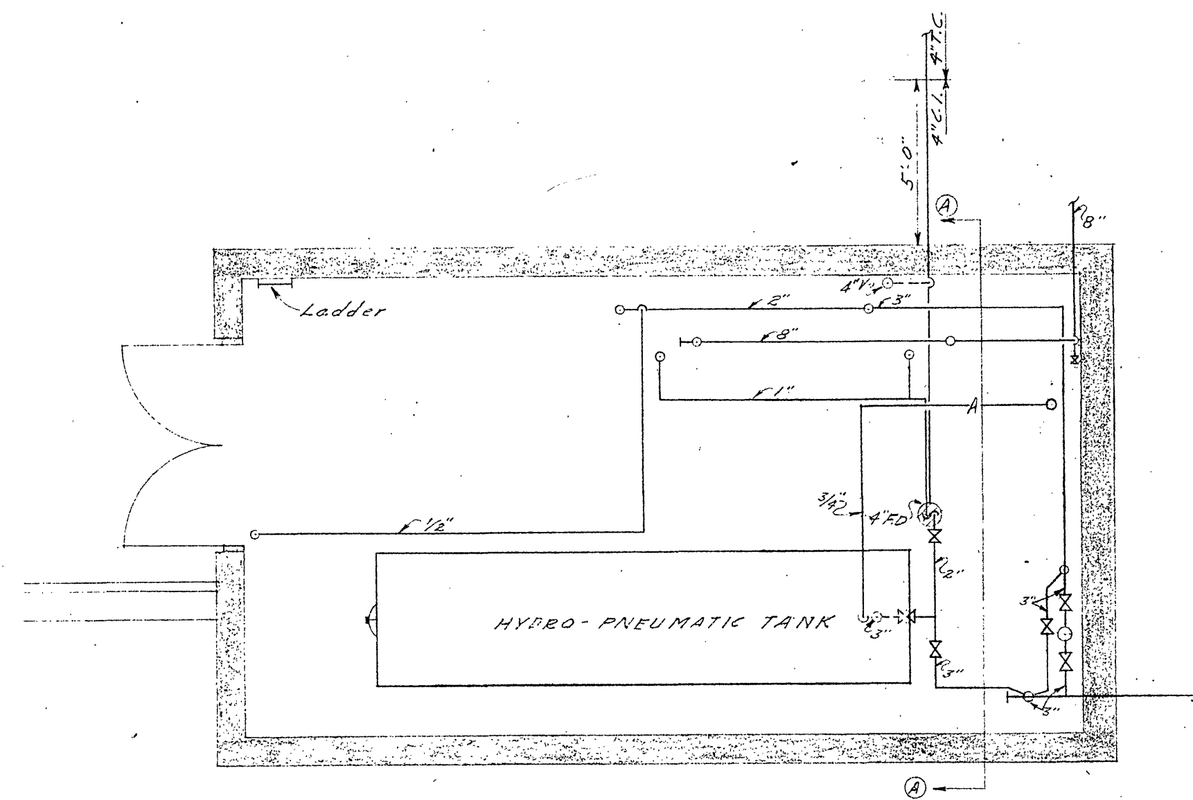
PLAN OF TANK ROOM SCALE: 1/4" = 1'-0"
