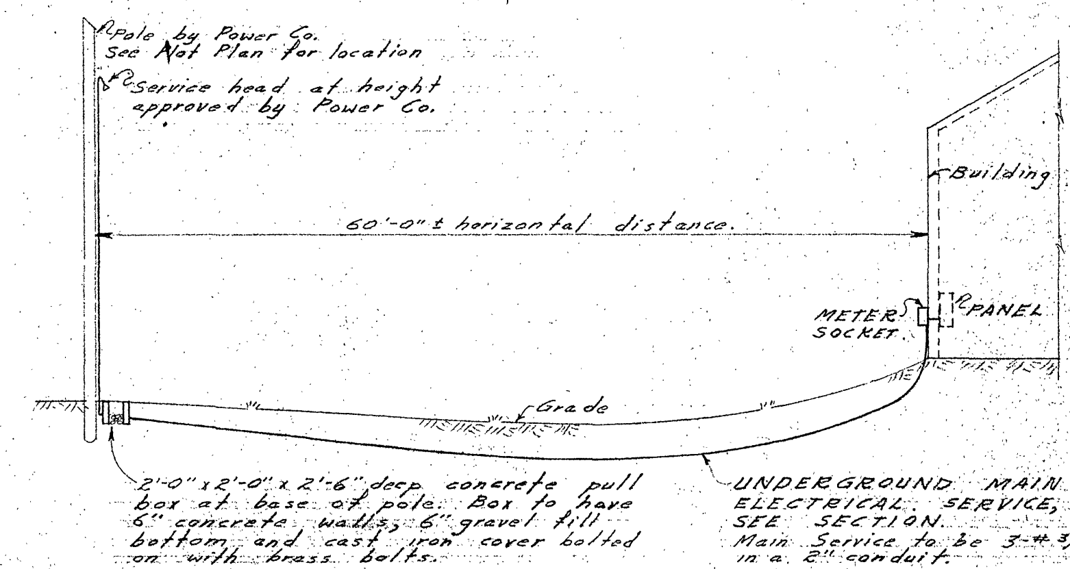
DETAIL OF MAIN SERVICE NO SCALE
