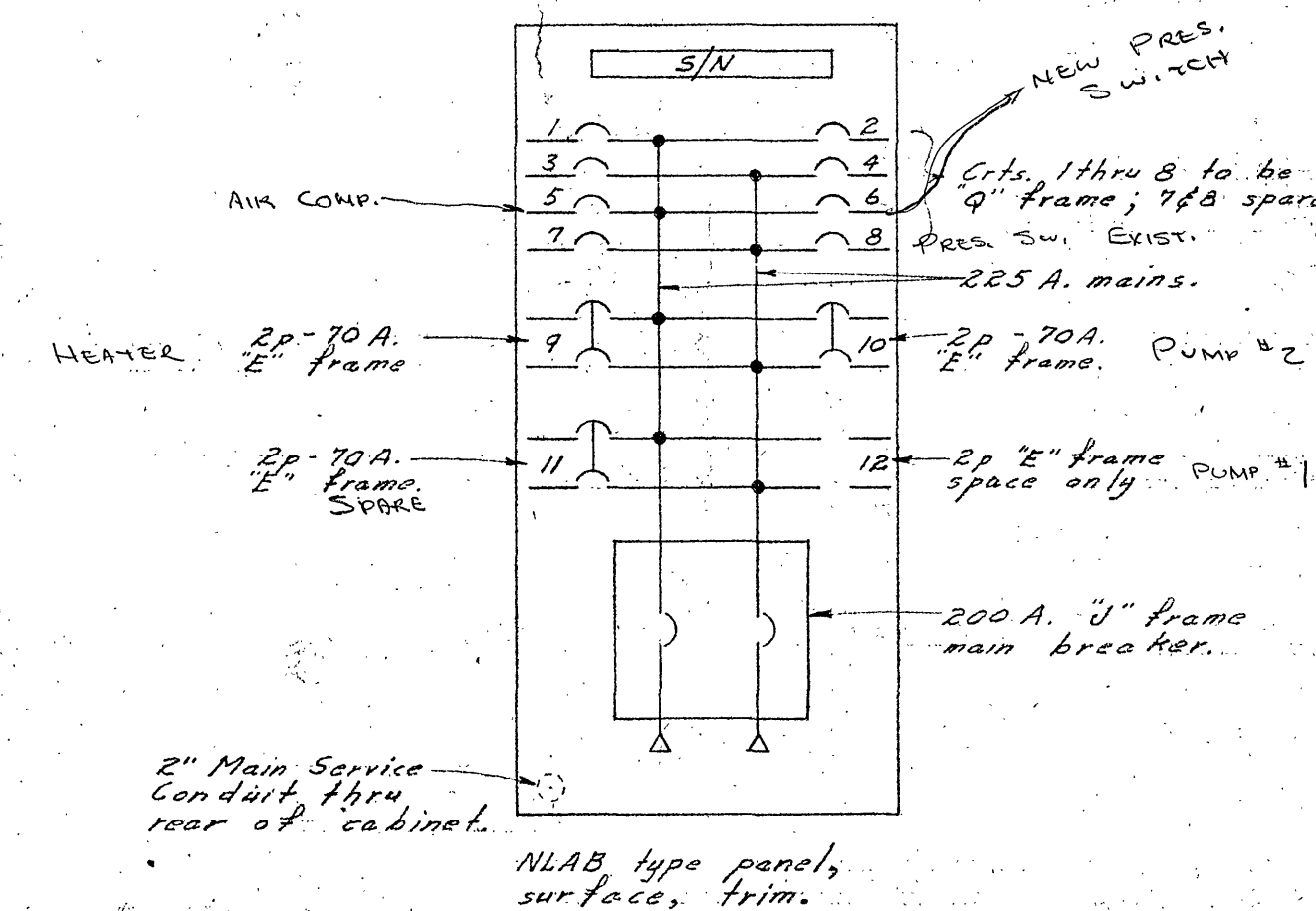
DETAIL OF PANEL-A NO SCALE
