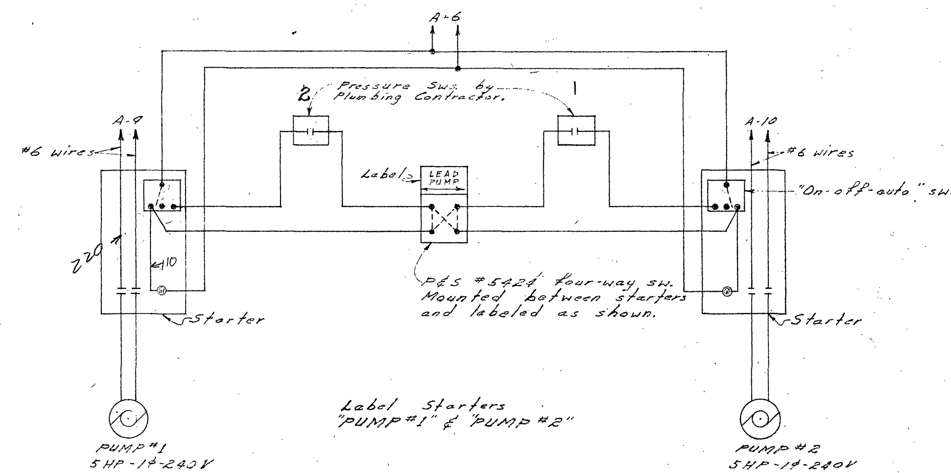
SCHEMATIC DIAGRAM OF PUMP #1 & #2 WIRING NO SCALE
