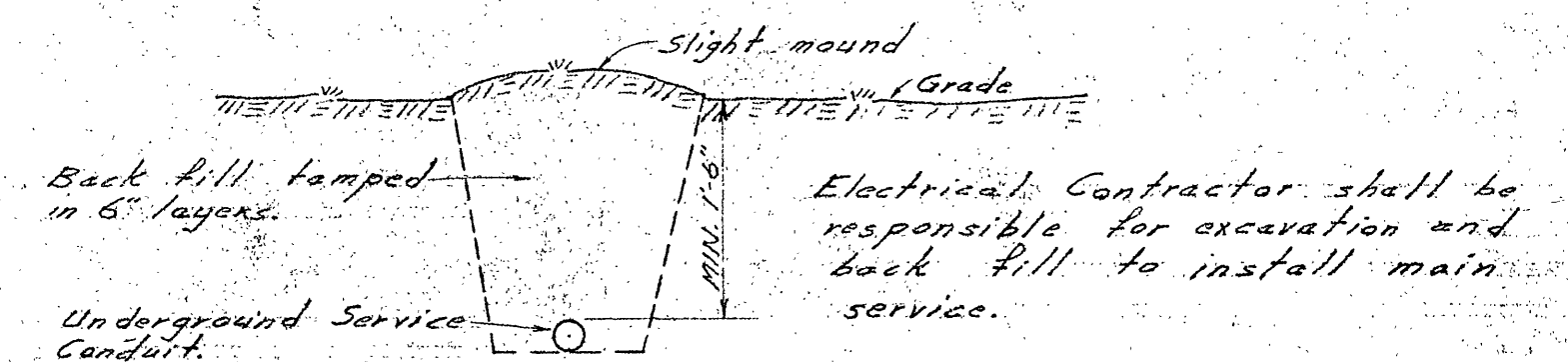
SECTION THROUGH UNDERGROUND SERVICE NO SCALE
