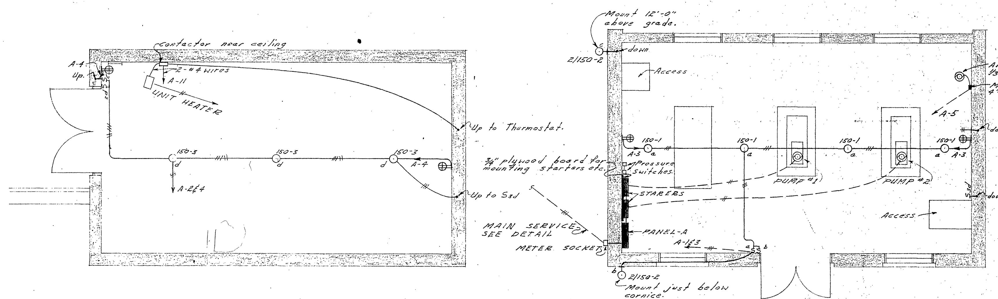
PLAN OF TANK ROOM SCALE: 1/4" = 1'-0"
