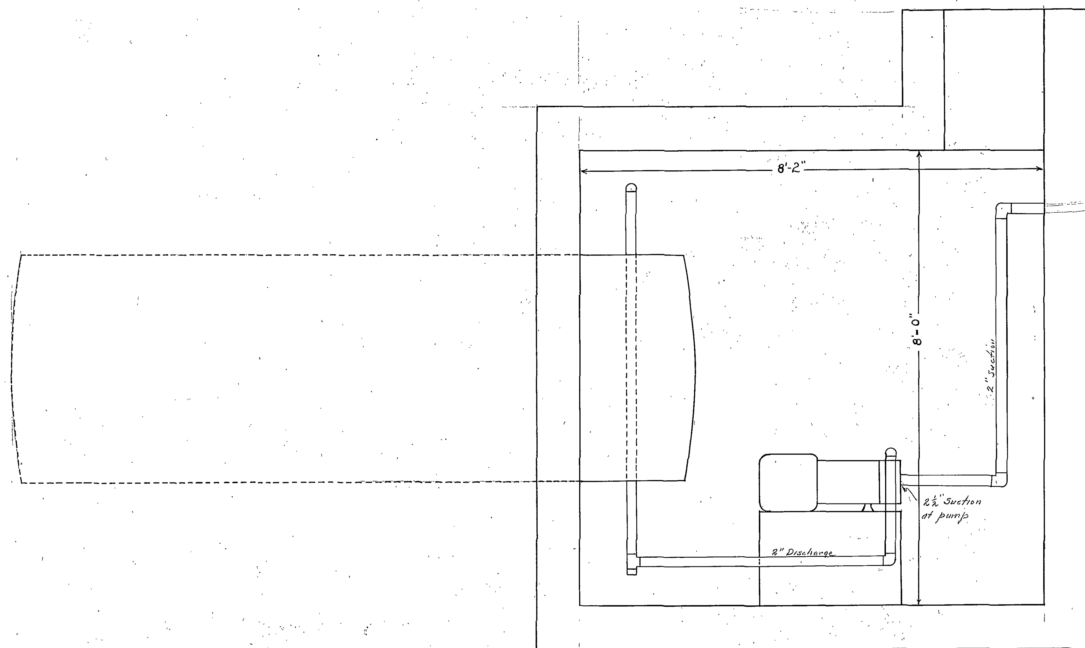
SECTION AA
