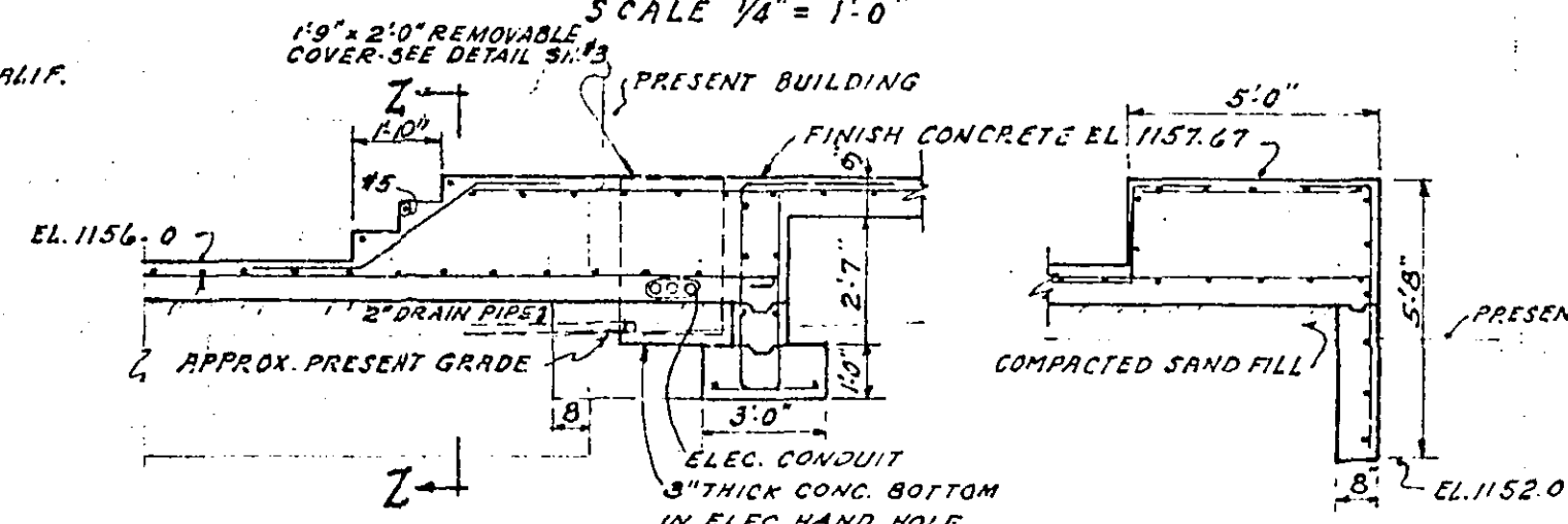
SECTION Y-Y
