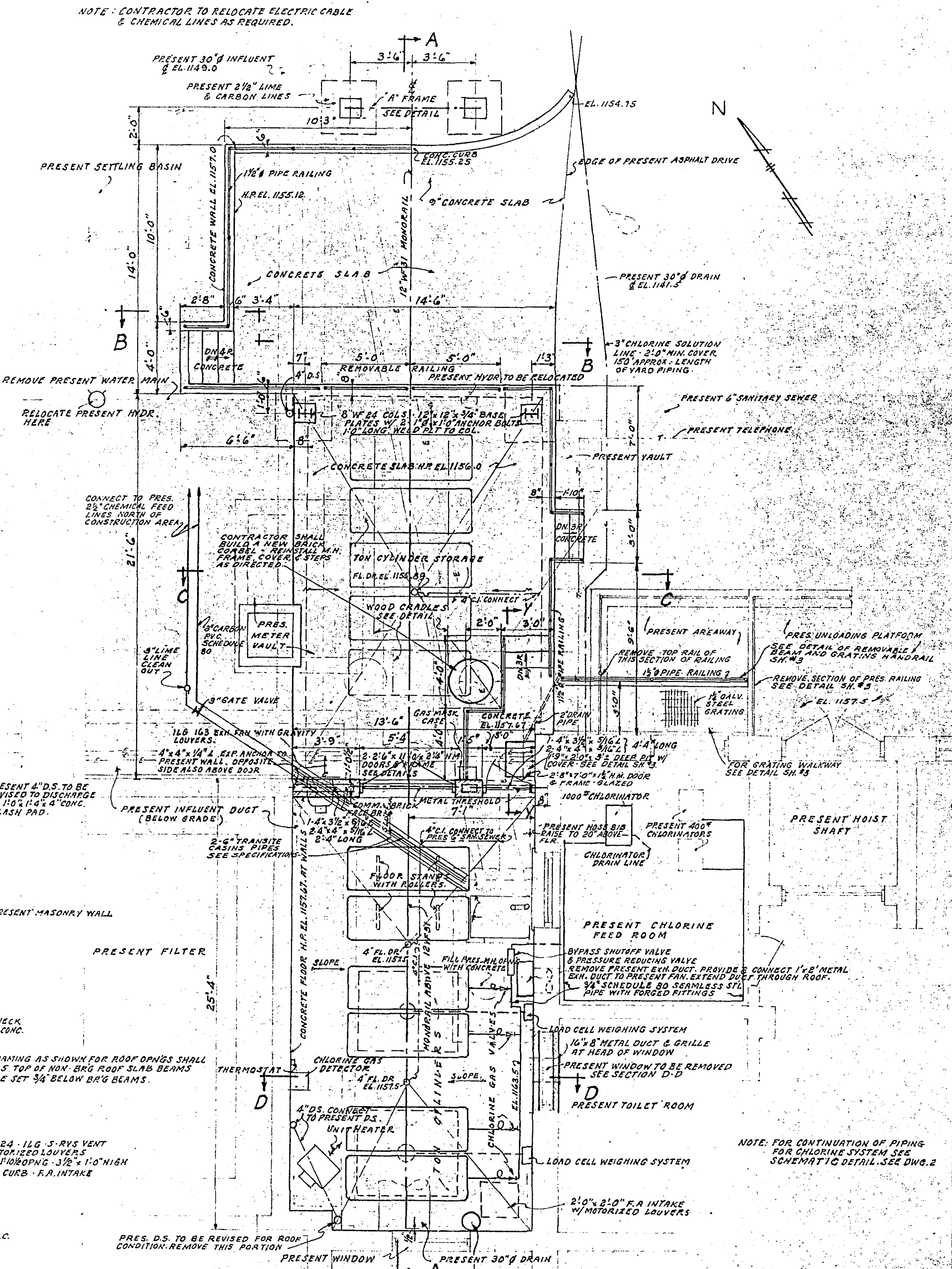
FLOOR PLAN
