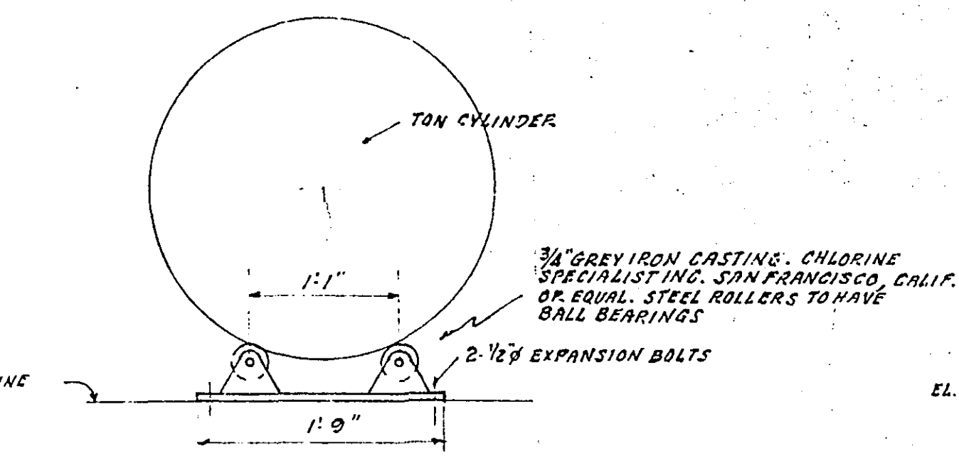
ROLLER CYLINDER CRADLE
