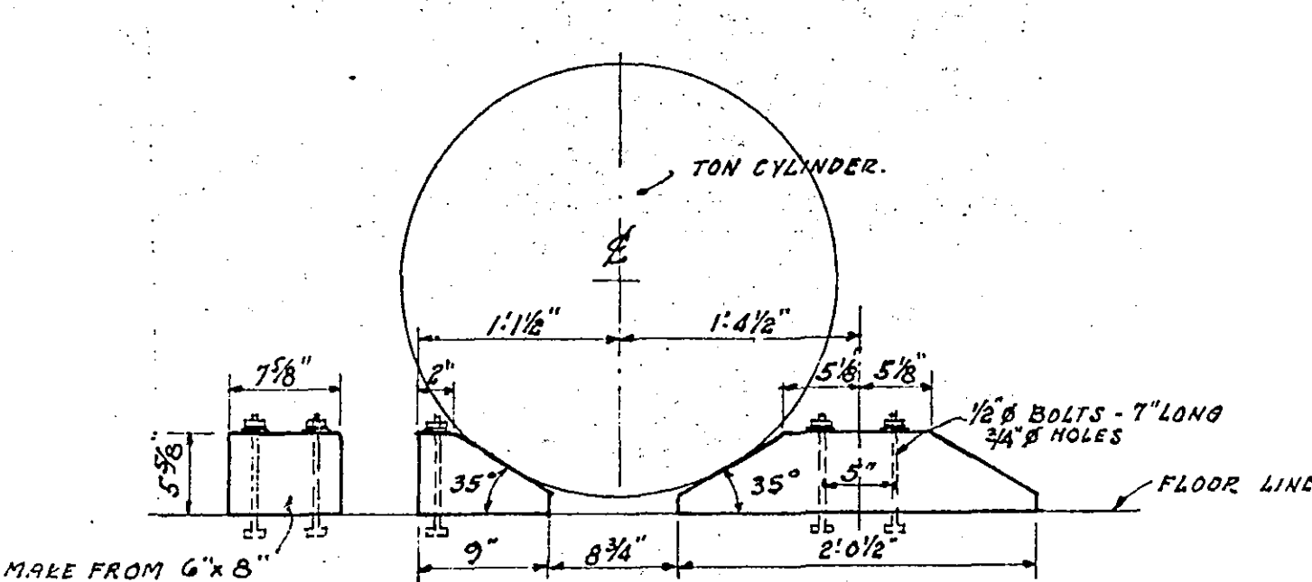
WOOD CRADLES DETAIL
