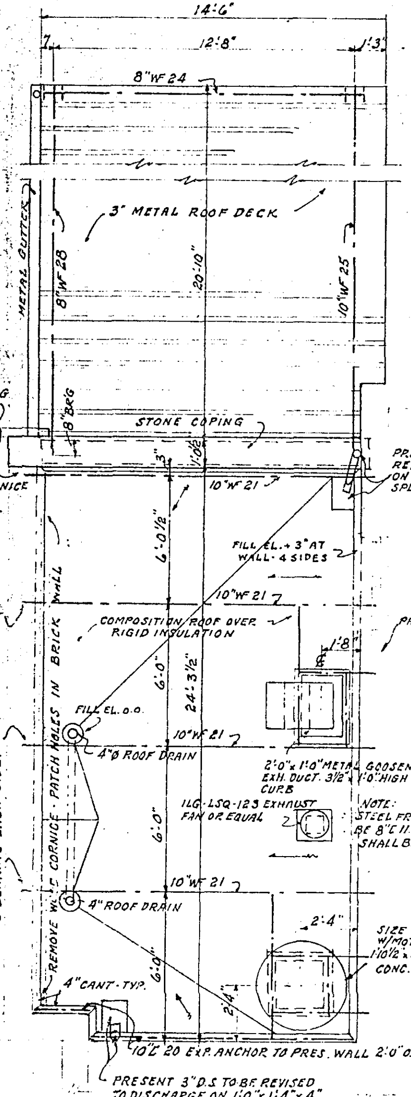
ROOF & ROOF FRAMING PLAN
