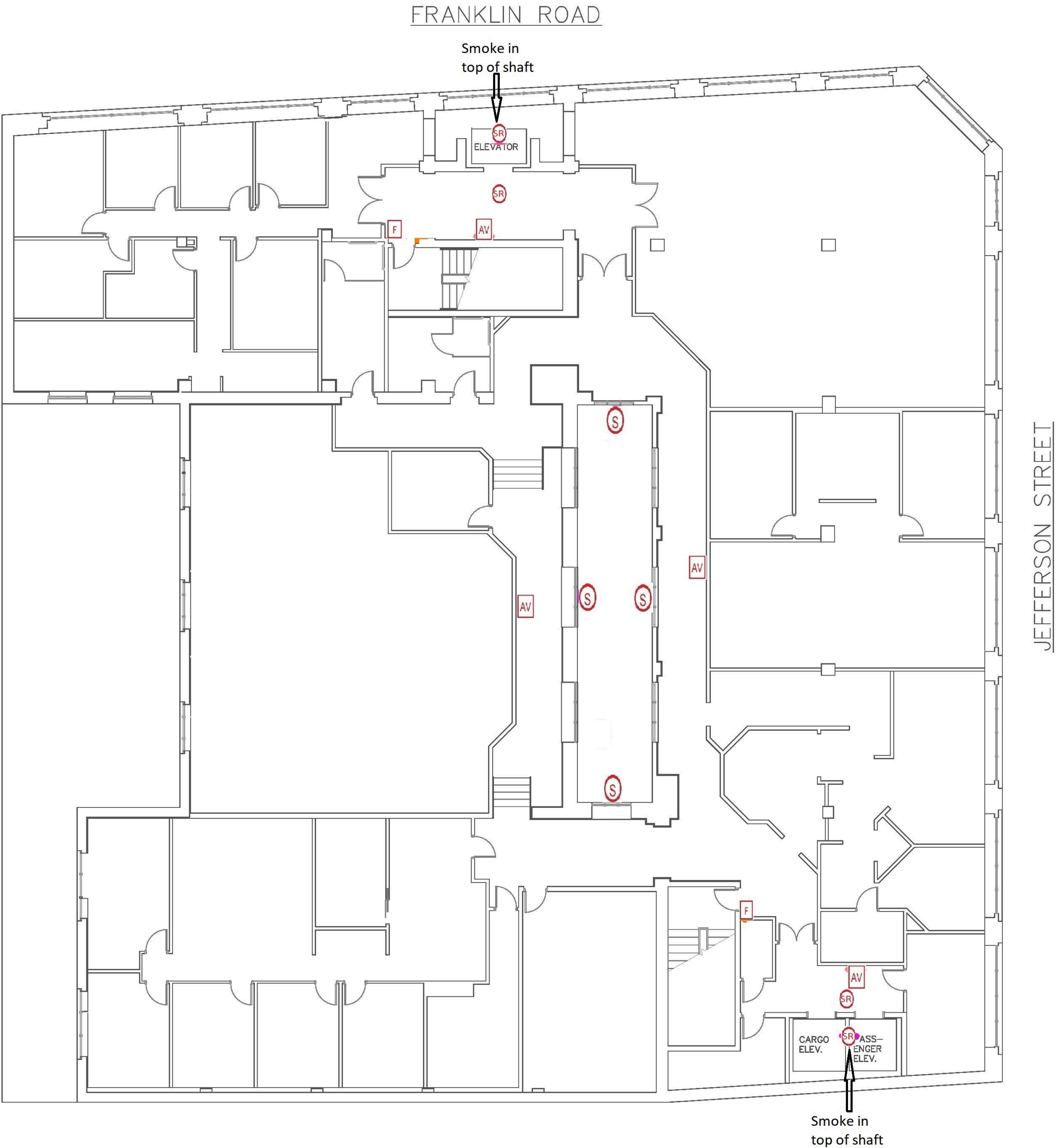
FOURTH FLOOR PLAN SCALE: 1/8" = 1'-0"
