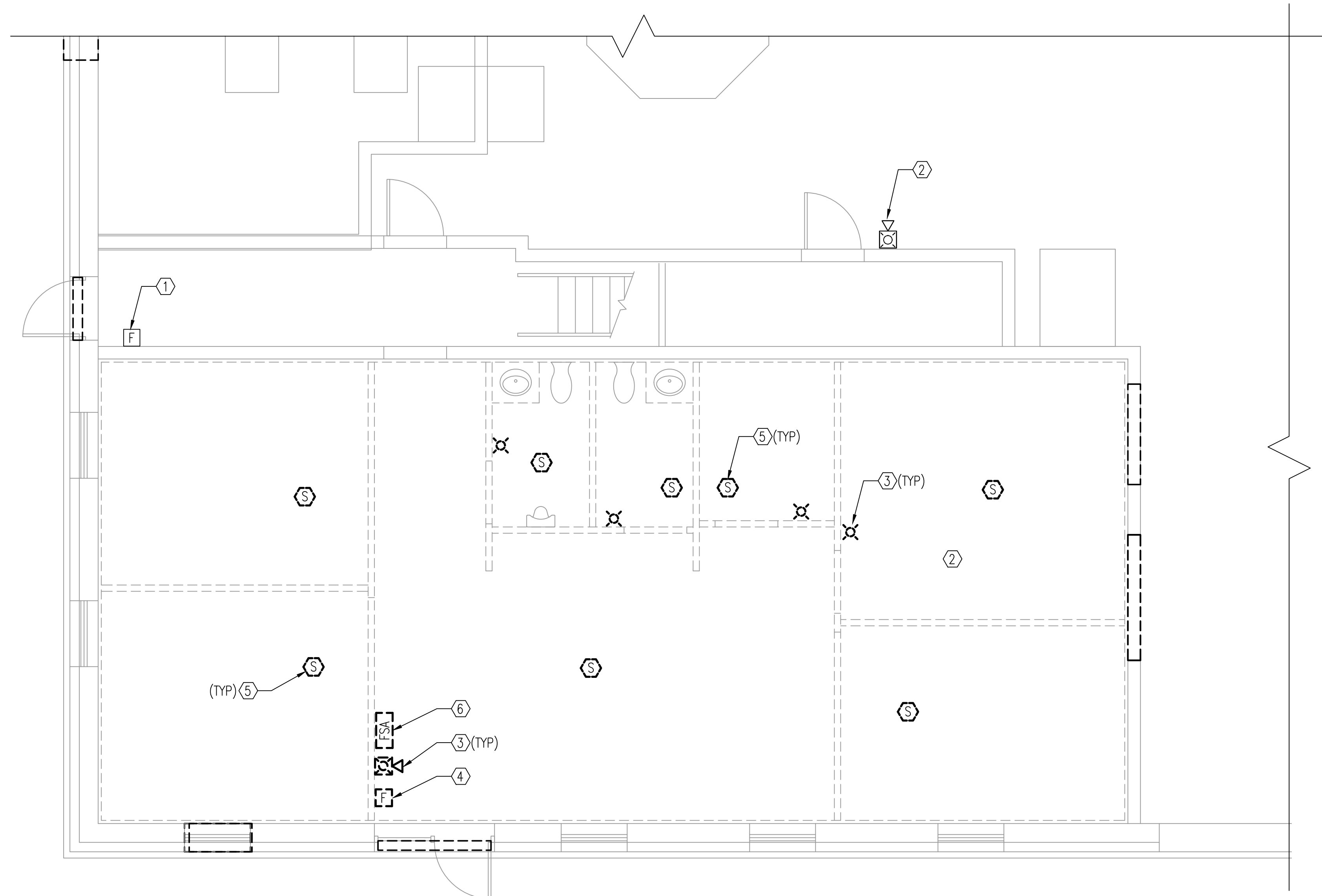
FIRE ALARM FLOOR PLAN - DEMOLITION SCALE: 1/4" = 1'-0"
