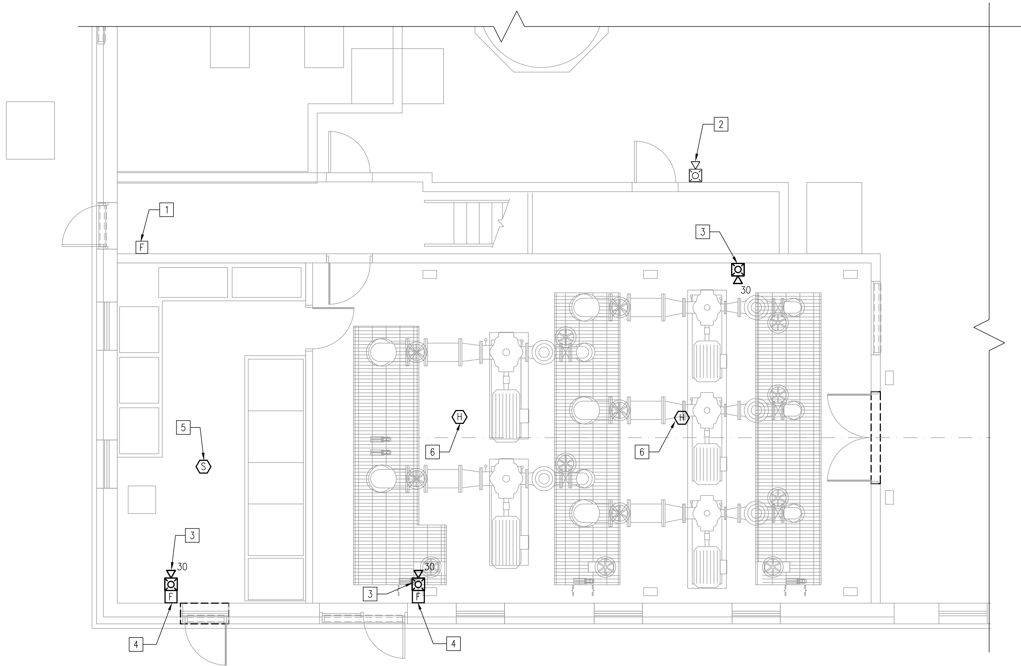
FIRE ALARM FLOOR PLAN - NEW WORK SCALE: 1/4" = 1'-0"
