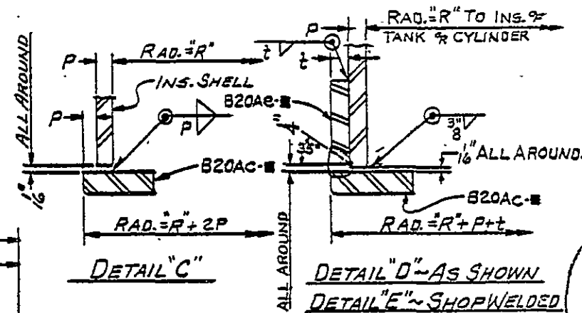
CRAB CLAMP DETAIL BEFORE FORMING-MK. B20Ad
