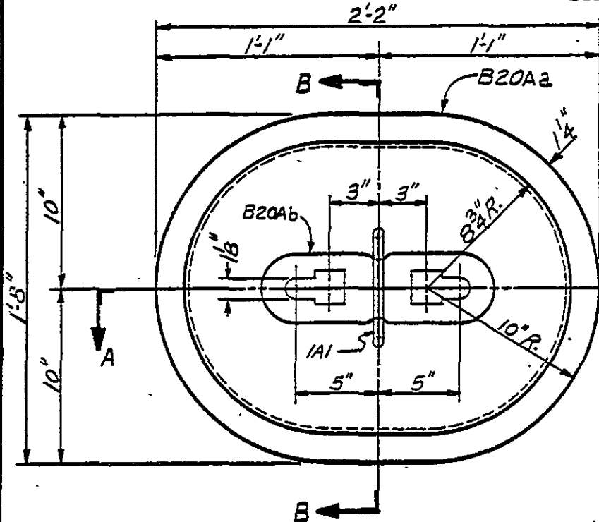
ELEVATION VIEW OF COVER
