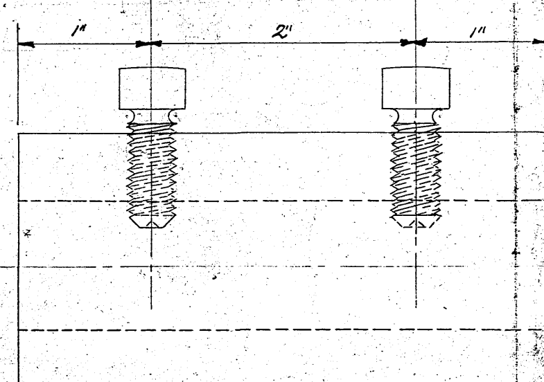
DETAIL- TYPICAL VALVE ROD GUIDE Scale Full
