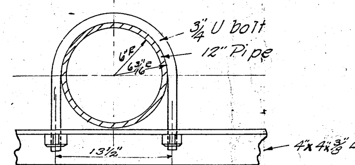
DETAIL- TYPICAL CLAMP FOR PIPE Scale 1"=18"
