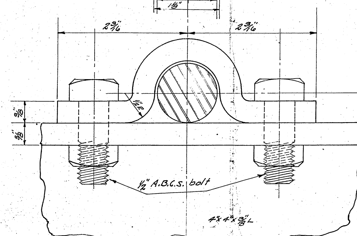
DETAIL- TYPICAL VALVE ROD GUIDE Scale Full
