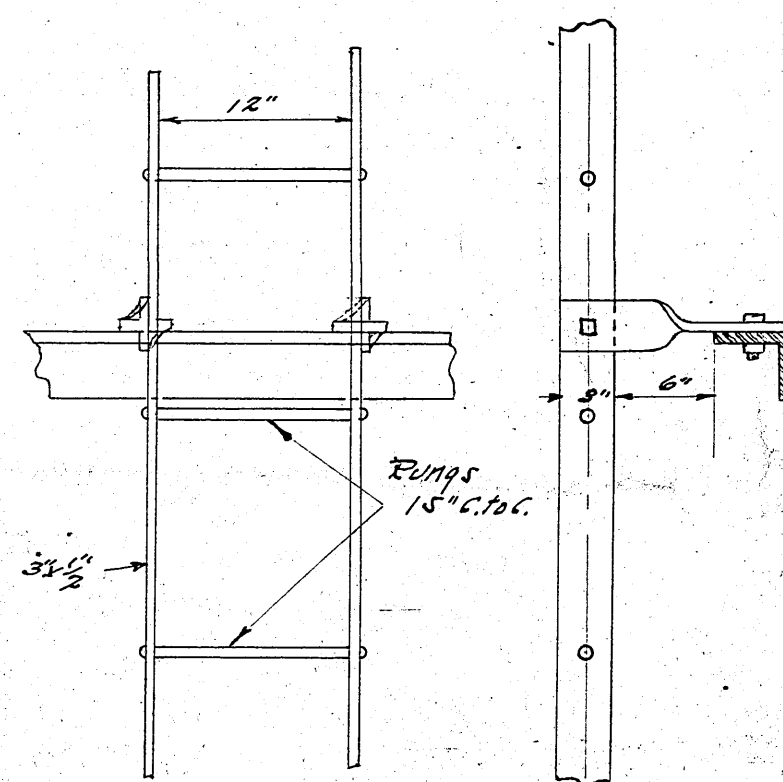
DETAIL- LADDER Scale 1"=1'
