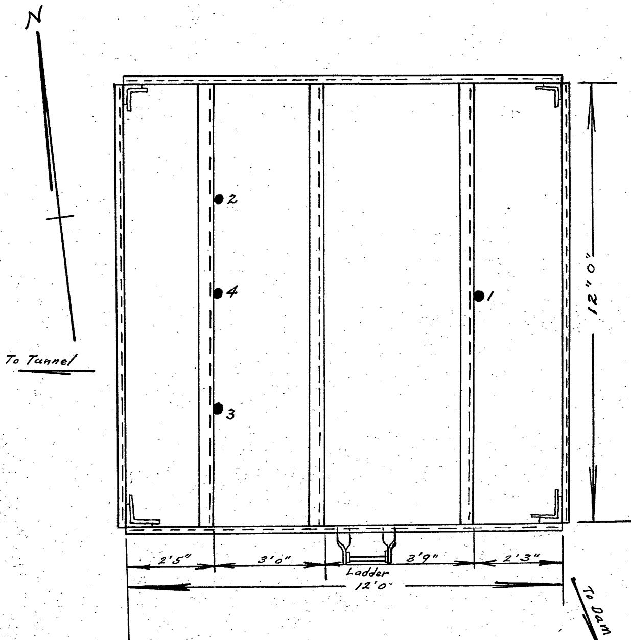
PLAN INTAKE TOWER BEAVER DAM CREEK (TOWER AT TUNNEL)
