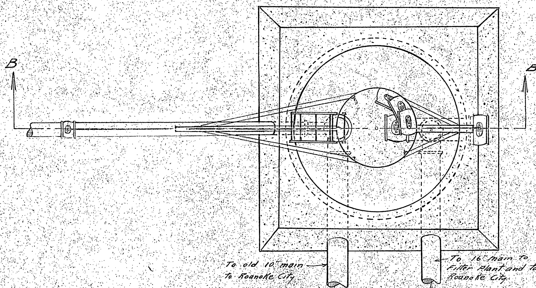
PROJECTION ON HORIZONTAL PLANE VIEW - A-A
