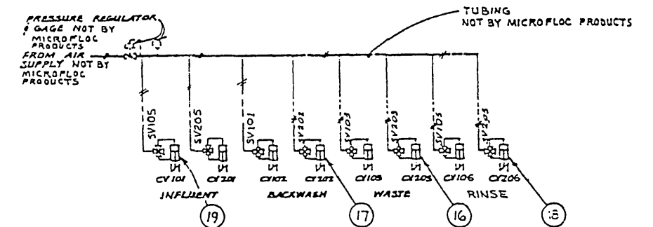
CONTROL VALVE AIR PIPING SCHEMATIC ISOLATION VALVE RECOMMENDED AT EL BRANCH CONNECTION
