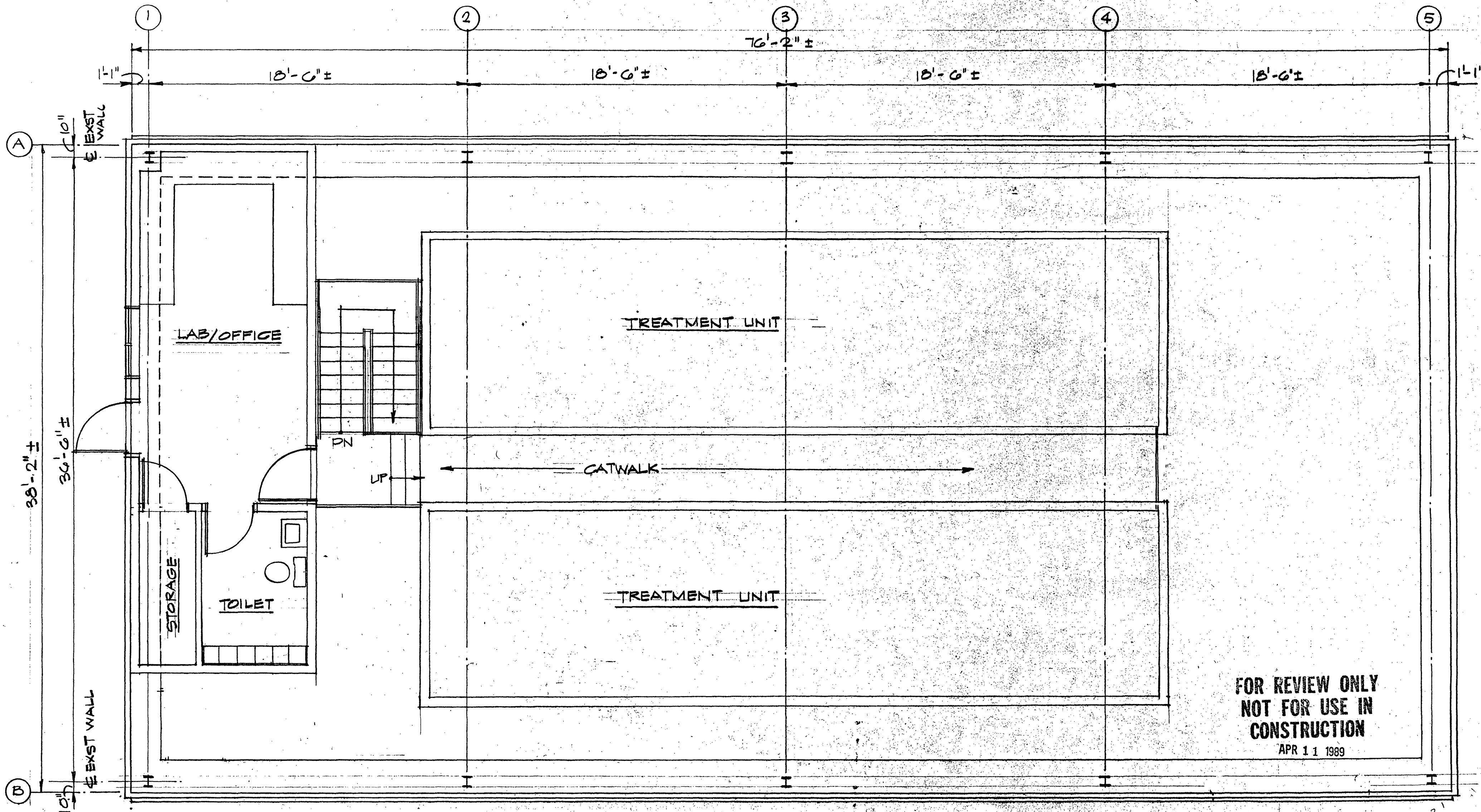
FILTER BLDG - UPPER LEVEL SCALE: 1/4" = 1'-0"
