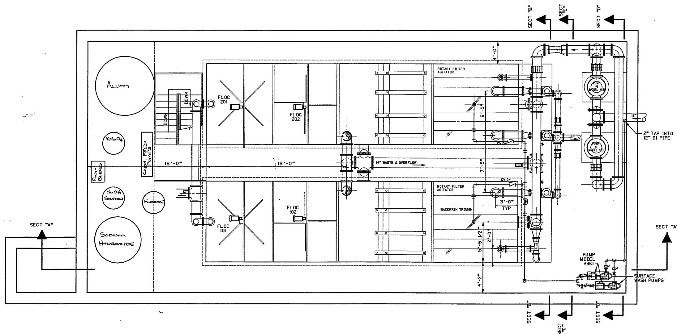
FLOOR PLAN SCALE: 1/4"=1'-0"
