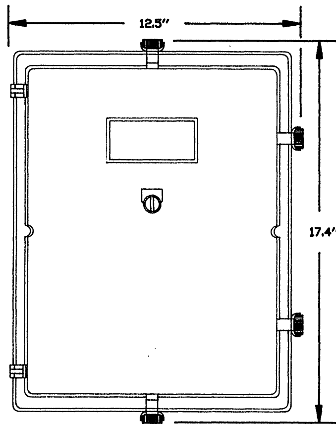
FRONT VIEW SCALE: 1/4" = 1" TAG: ENC-1
