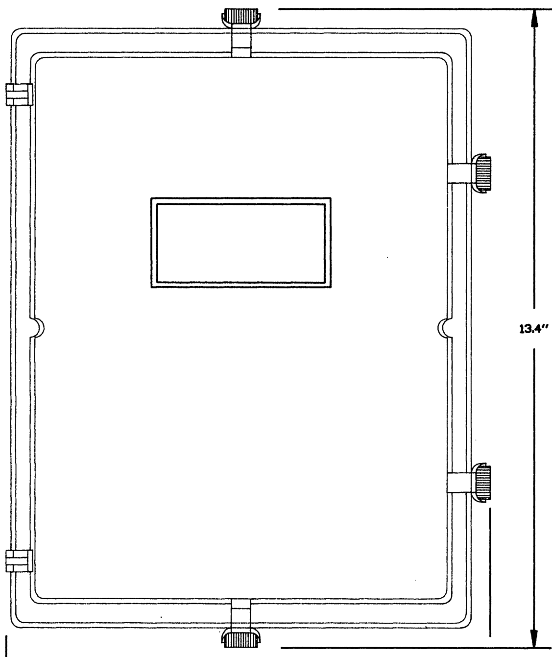
FRONT VIEW SCALE: 1/2" = 1" TAG: ENC-1
