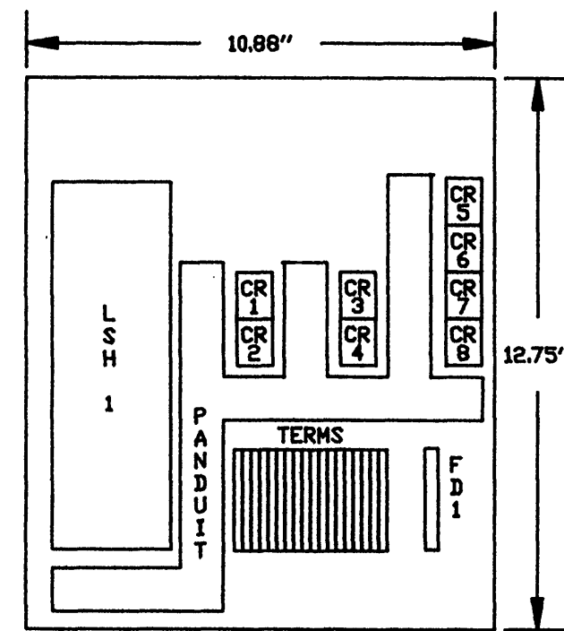
BACK PANEL SCALE: 1/4" = 1" TAG: BACKPAN
