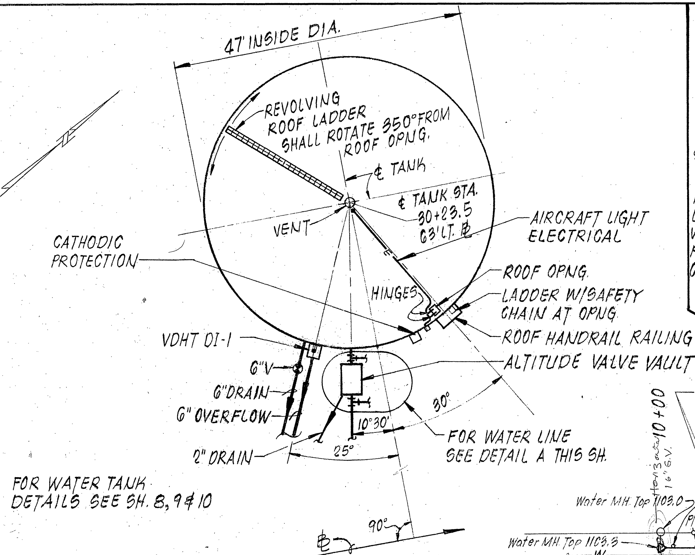
WATER TANK ROOF PLAN NO SCALE
