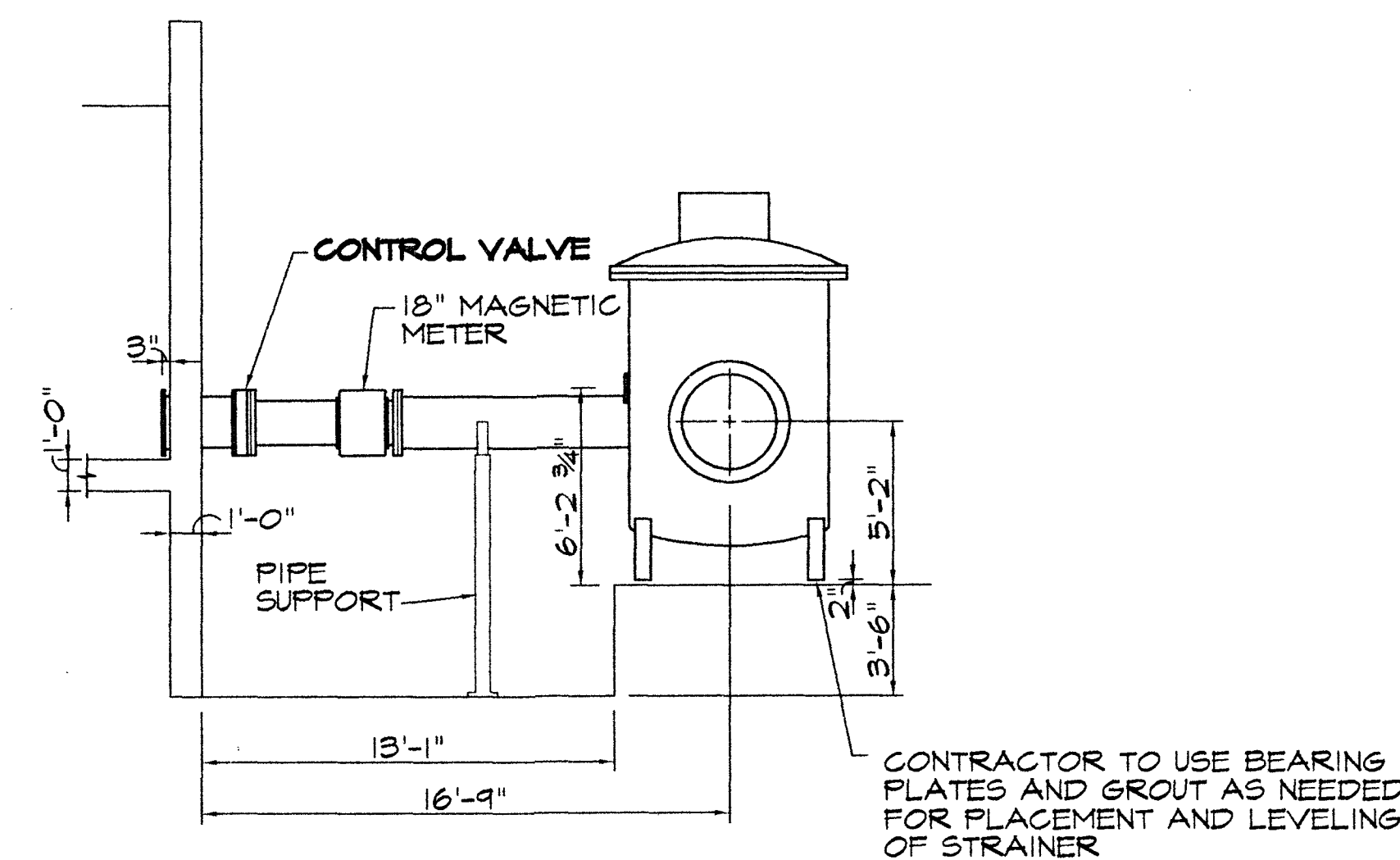
SECTION DETAIL - RAW / STRAINER
