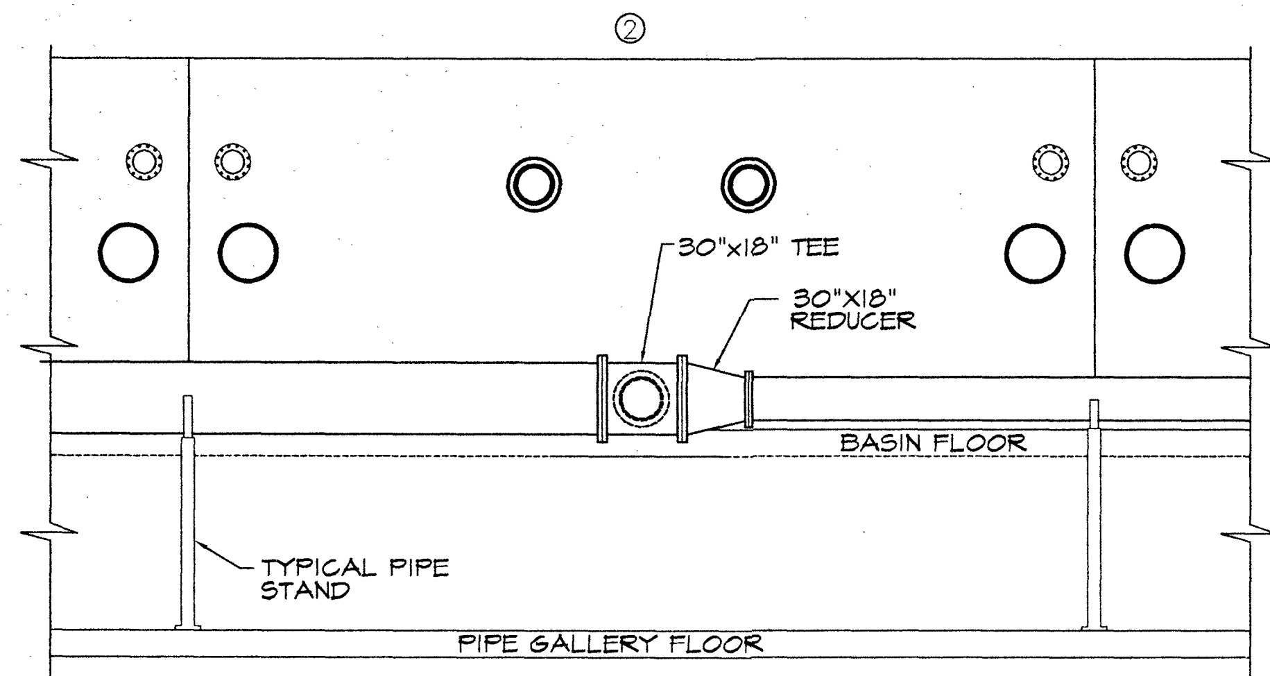
BASIN #2 - RAW WATER PIPING ELEVATION
