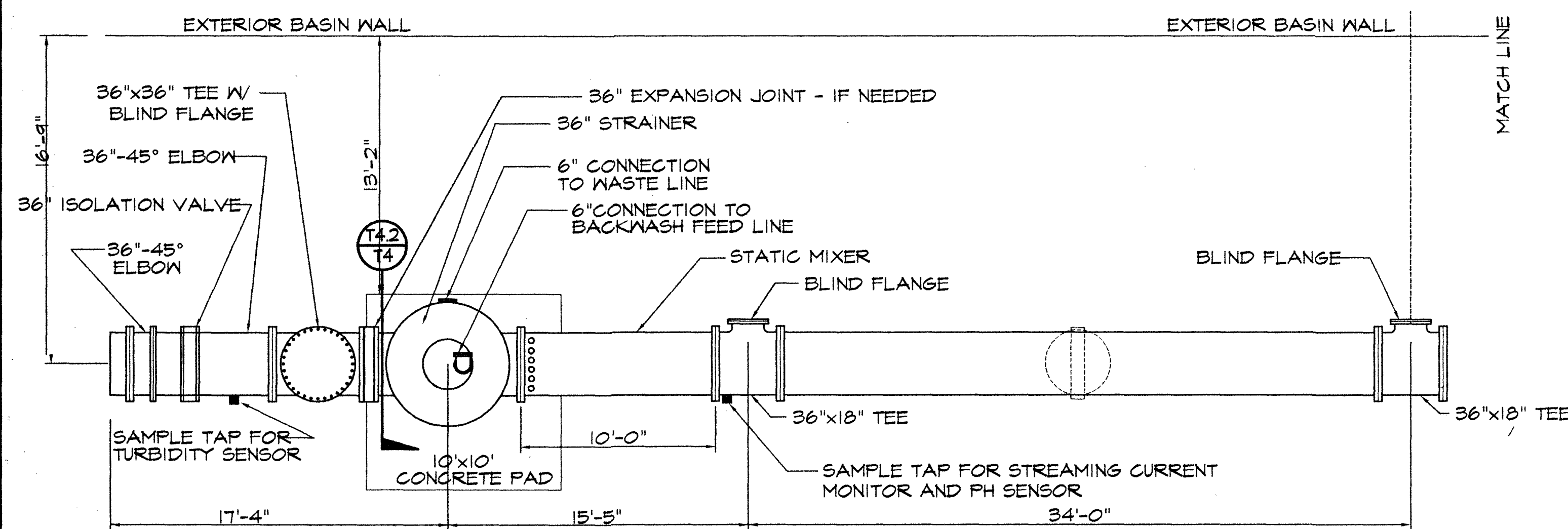
RAW WATER PIPING PLAN
