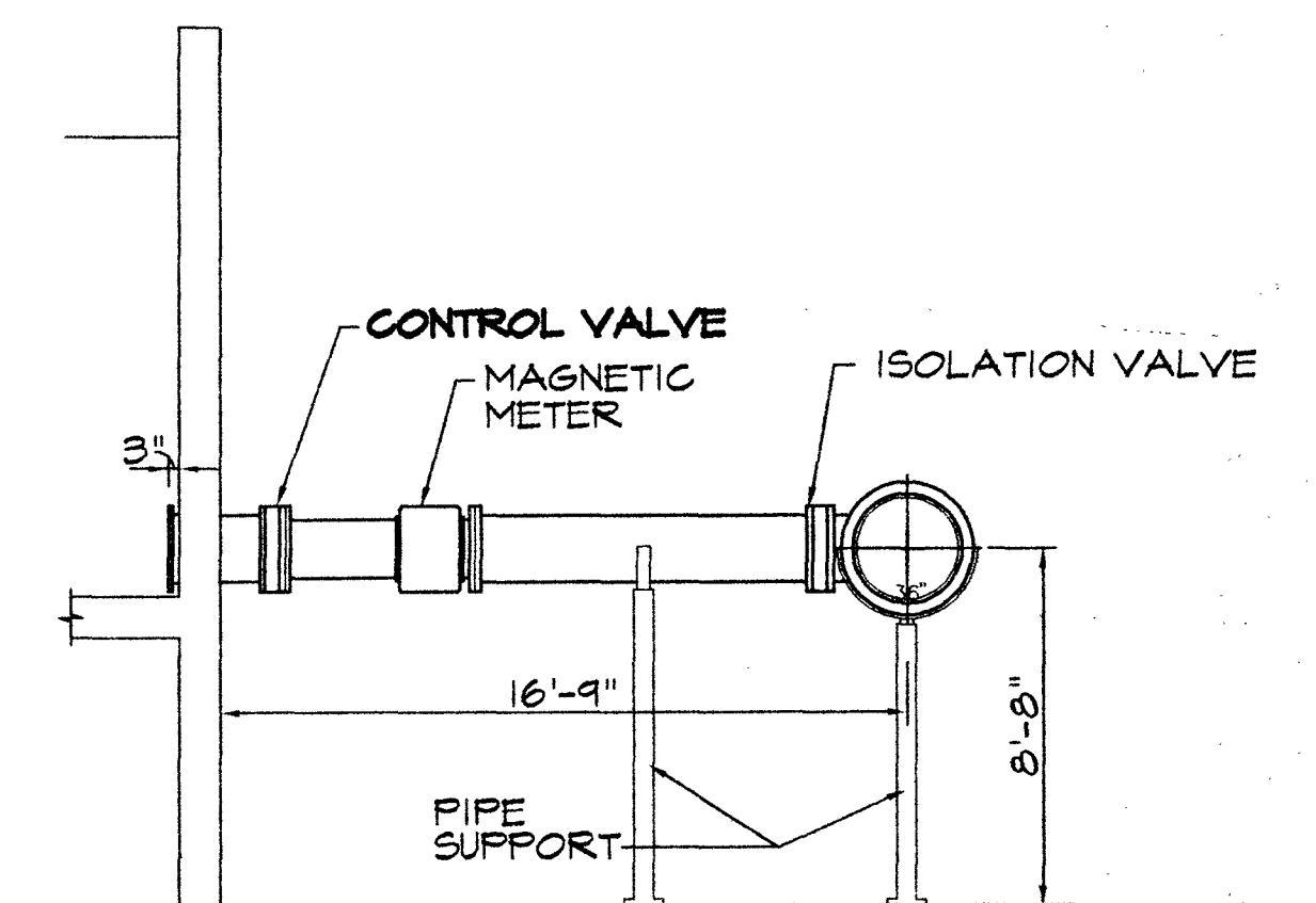
SECTION DETAIL - RAW
