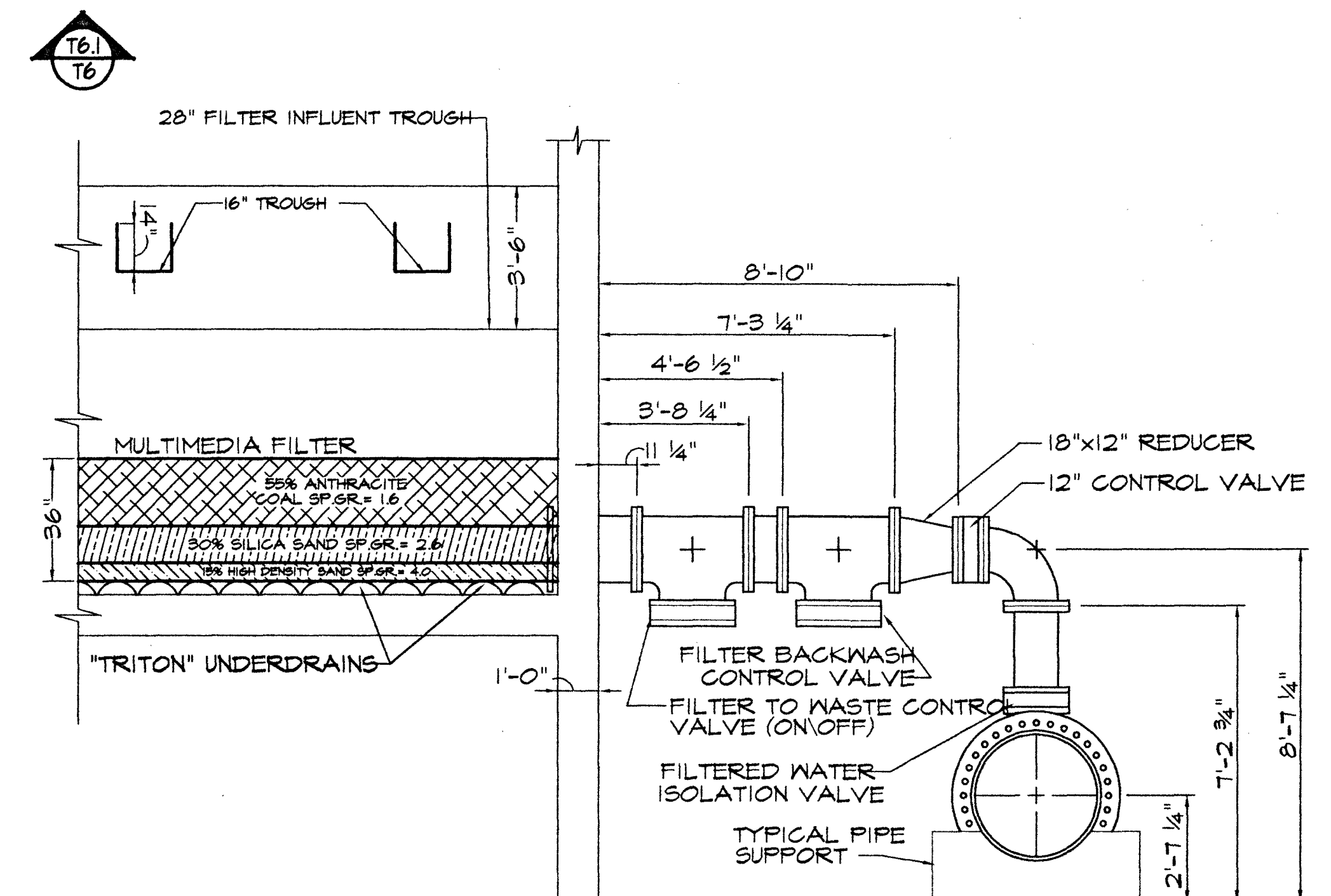
SECTION - FILTERED SCALE 1" = 3'-0"
