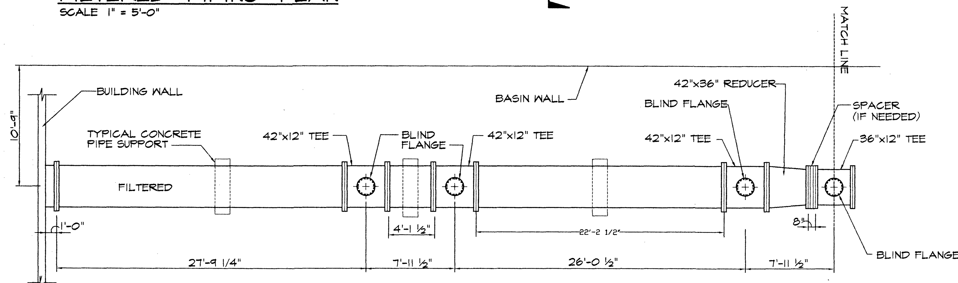
FILTERED PIPING PLAN SCALE 1" = 5'-0"
