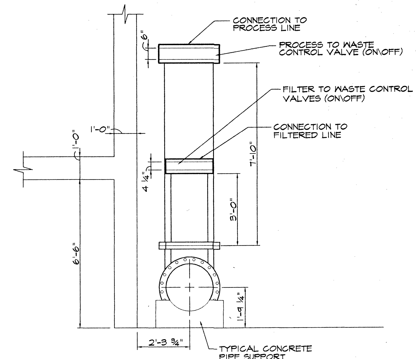
WASTE PIPING SECTION SCALE 1" = 2'-0" • OUTSIDE BUILDING WALL
