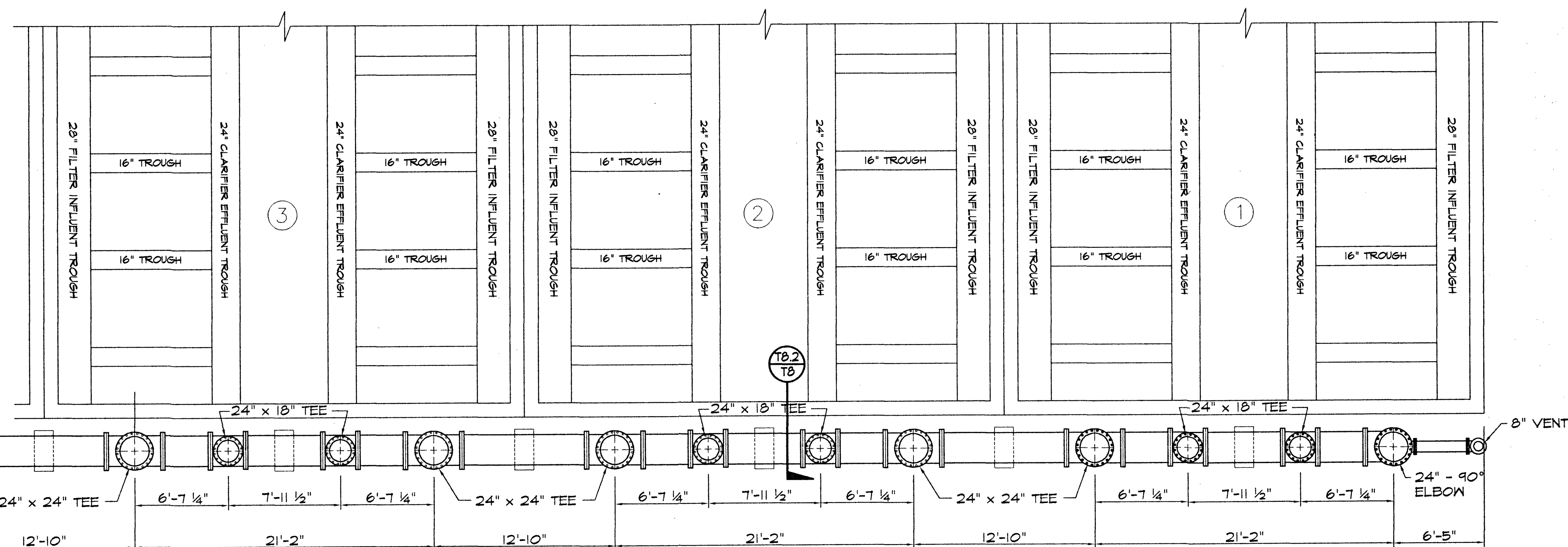
WASTE PIPING PLAN SCALE 1" = 5'-0"
