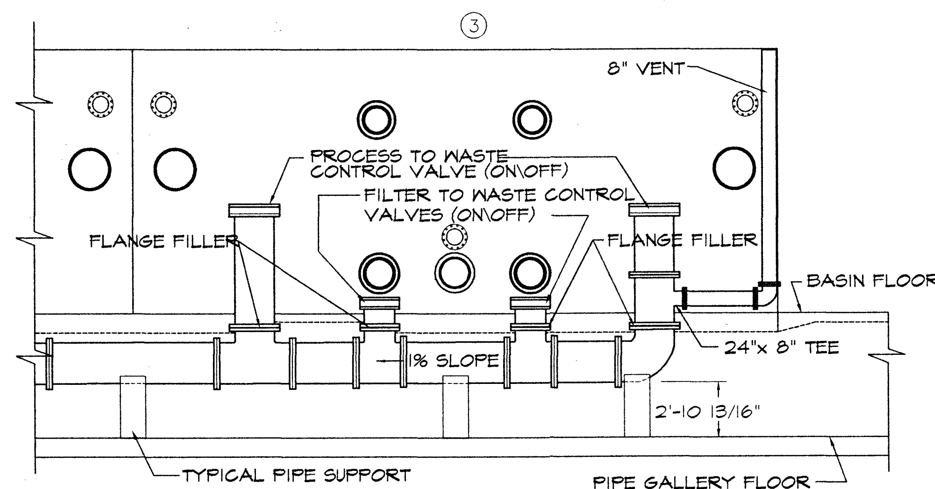
BASIN #3 - WASTE PIPING ELEVATION SCALE 1" = 5'-0"
